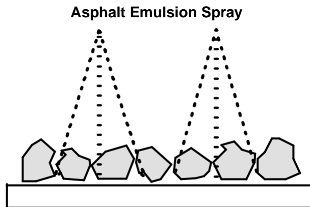
Figure 1: Schematic of Fog Seal Application
