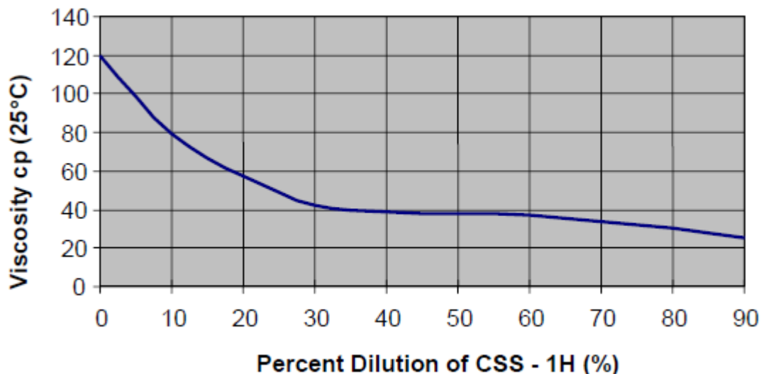
Figure 8: Viscosity Change with Dilution
