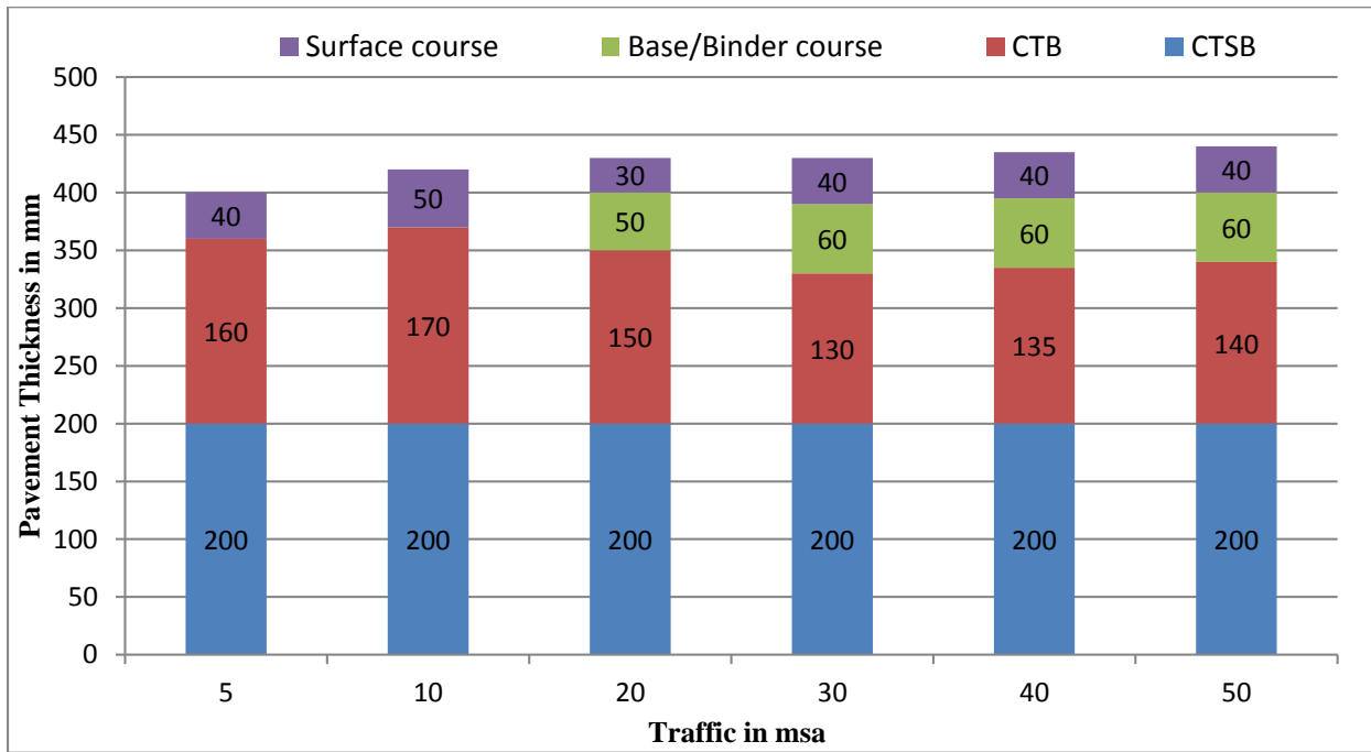
Figure 12.21 Catalogue for pavement with bituminous surface course with CTSB, CTB and SAMI - Effective CBR 9% (Plate-21)
