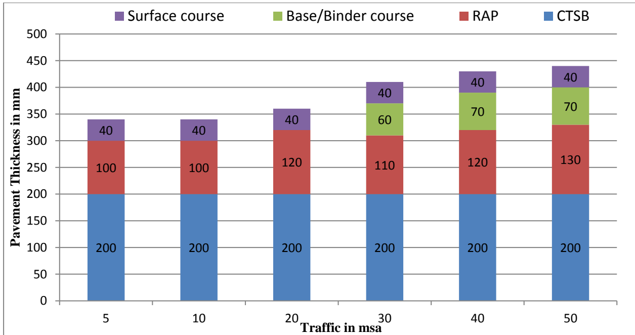
Figure 12.26 Catalogue for pavement with bituminous surface course with CTSB and emulsion/foam bitumen stabilised RAP/virgin aggregate - Effective CBR 6% (Plate-26)
