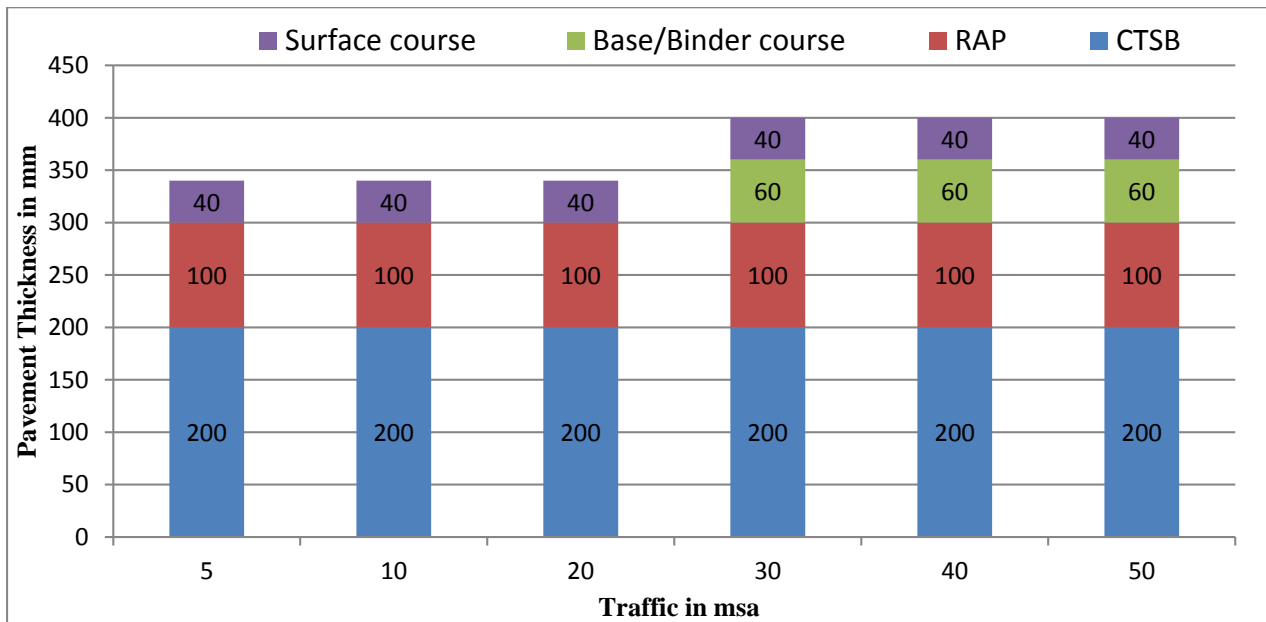
Figure 12.31 Catalogue for pavement with bituminous surface course with CTSB and emulsion/foam bitumen stabilised RAP/virgin aggregate - Effective CBR 12% (Plate-31)
