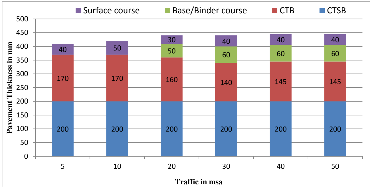
Figure 12.18 Catalogue for pavement with bituminous surface course with CTSB, CTB and SAMI - Effective CBR 6% (Plate-18)
