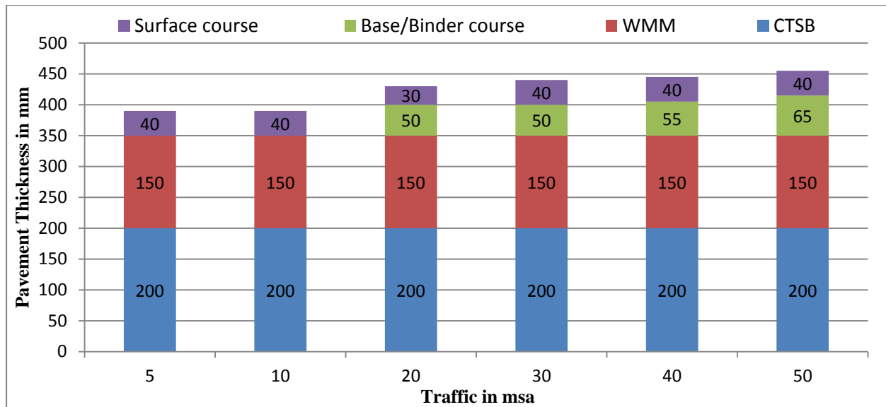
Figure 12.48 Catalogue for pavement with bituminous surface course with CTSB and granular base course - Effective CBR 15% (Plate-48)
