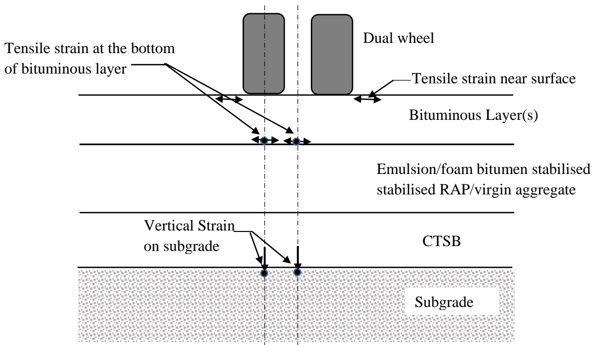
Figure 3.4 A pavement section with bituminous layer(s), emulsion/foam bitumen stabilised RAP/virgin aggregate layer and CTSB showing the locations of critical strains
