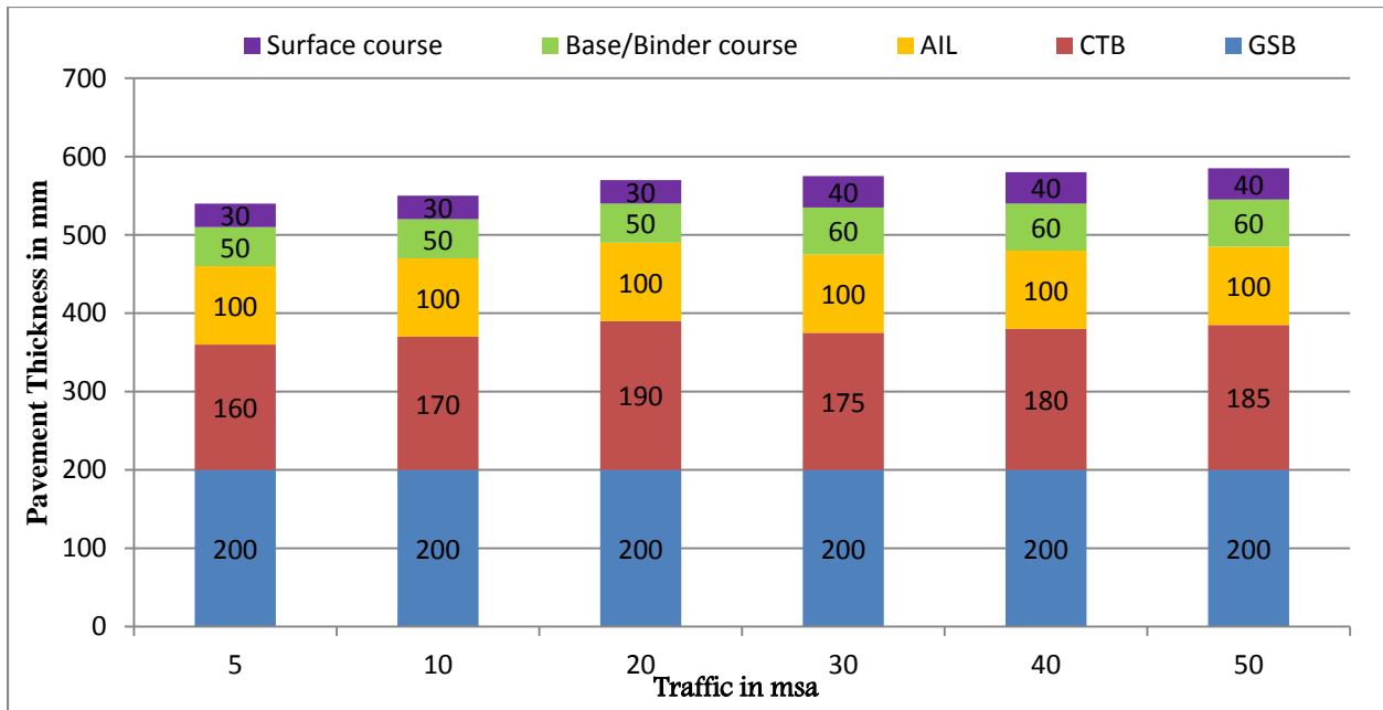
Figure 12.33 Catalogue for pavement with bituminous surface course with GSB, CTB and granular crack relief layer - Effective CBR 5% (Plate-33)
