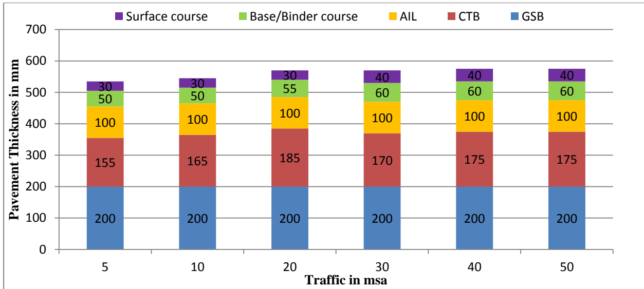
Figure 12.34 Catalogue for pavement with bituminous surface course with GSB, CTB and granular crack relief layer - Effective CBR 6% (Plate-34)
