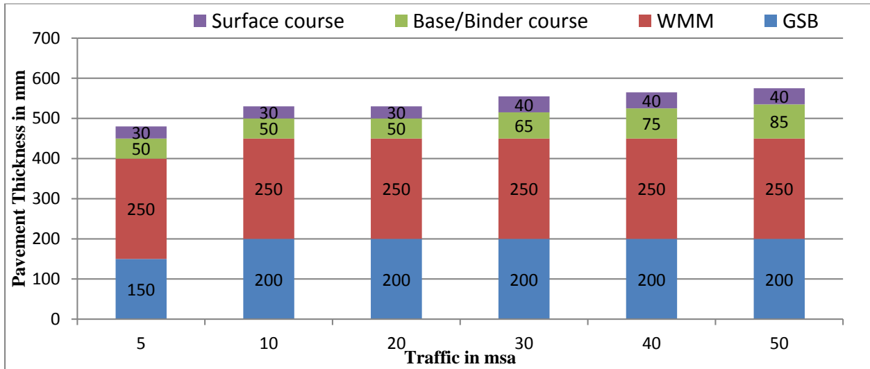
Figure 12.8 Catalogue for pavement with bituminous surface course with granular base and sub-base - Effective CBR 15% (Plate-8)
