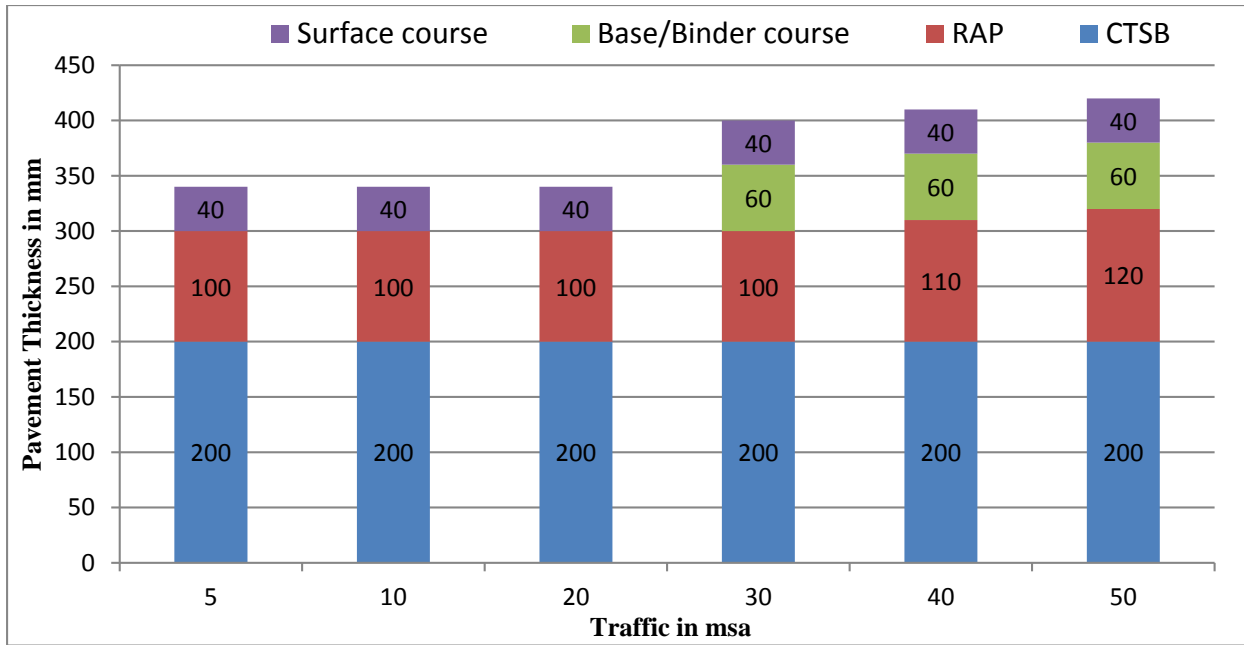
Figure 12.28 Catalogue for pavement with bituminous surface course with CTSB and emulsion/foam bitumen stabilised RAP/virgin aggregate - Effective CBR 8% (Plate-28)
