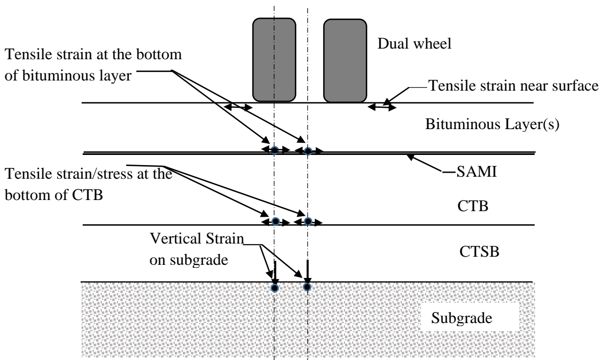
Figure 3.3 A pavement section with bituminous layer(s), SAMI crack relief layer, CTB, and CTSB showing the locations of critical strains
