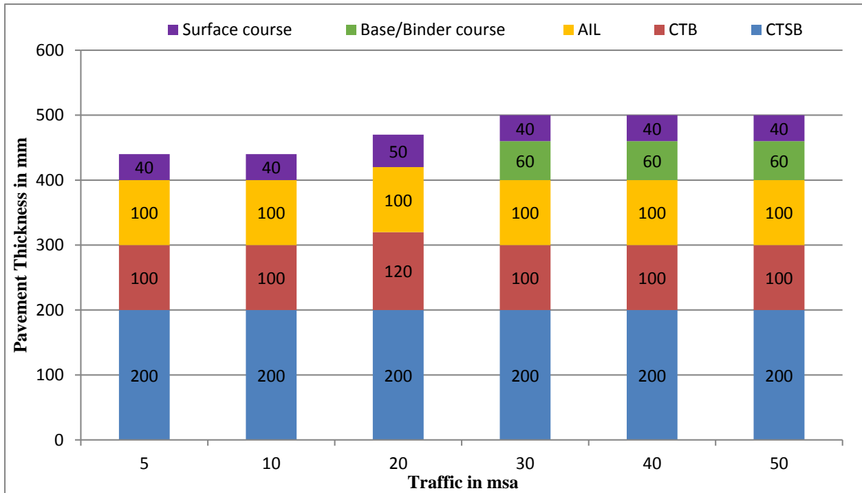
Figure 12.11 Catalogue for pavement with bituminous surface course with CTSB, CTB and granular crack relief layer - Effective CBR 7% (Plate-11)
