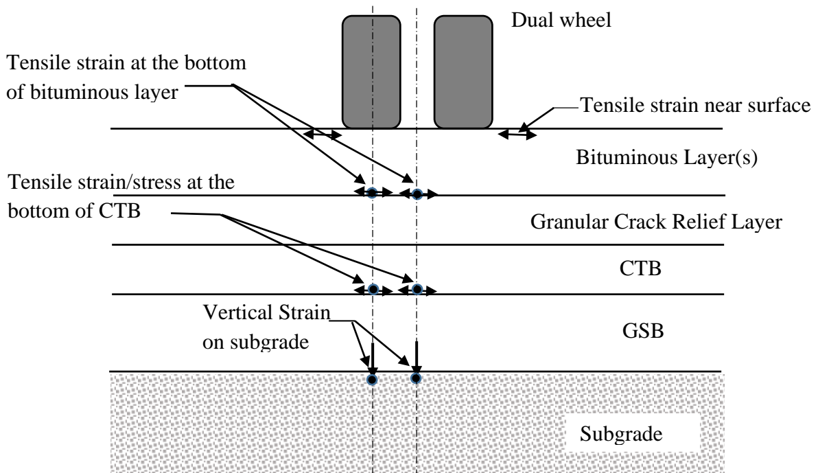
Figure 3.5 A pavement section with bituminous layer(s), granular crack relief layer, CTB, and GSB showing the locations of critical strains
