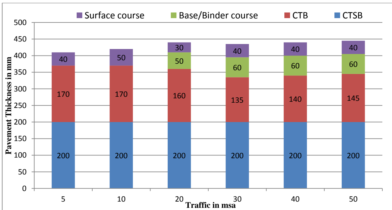
Figure 12.19 Catalogue for pavement with bituminous surface course with CTSB, CTB and SAMI - Effective CBR 7% (Plate-19)
