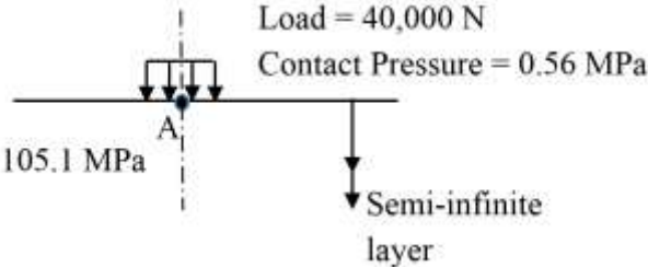
Figure II.2 Equivalent (effective) Subgrade System
