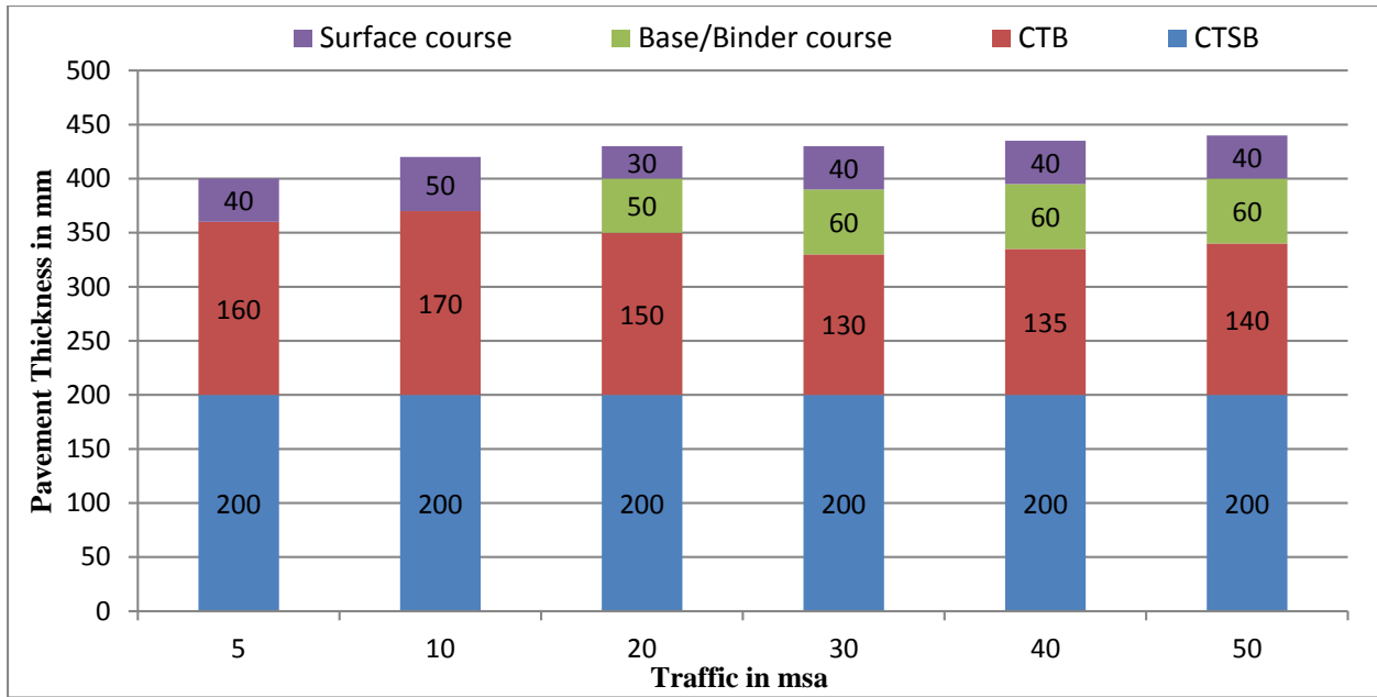
Figure 12.20 Catalogue for pavement with bituminous surface course with CTSB, CTB and SAMI - Effective CBR 8% (Plate-20)
