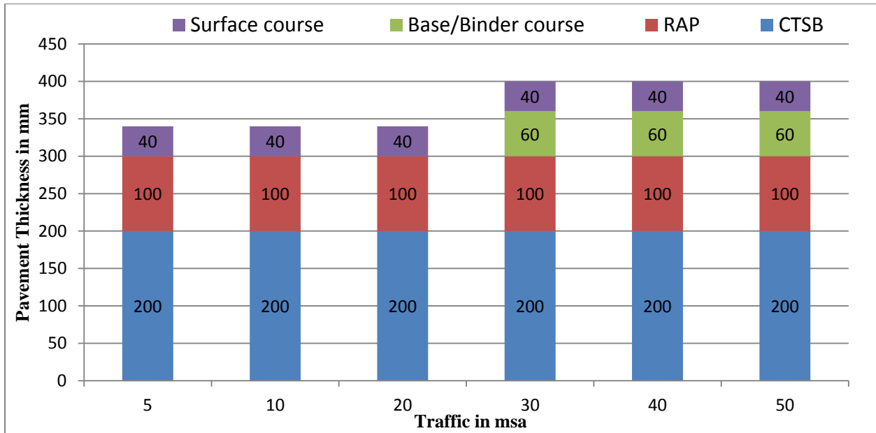
Figure 12.32 Catalogue for pavement with bituminous surface course with CTSB and emulsion/foam bitumen stabilised RAP/virgin aggregate - Effective CBR 15% (Plate-32)
