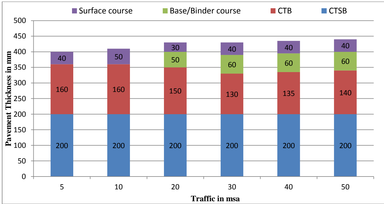
Figure 12.23 Catalogue for pavement with bituminous surface course with CTSB, CTB and SAMI - Effective CBR 12% (Plate-23)
