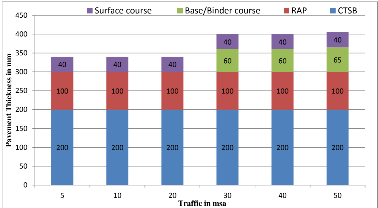
Figure 12.30 Catalogue for pavement with bituminous surface course with CTSB and emulsion/foam bitumen stabilised RAP/virgin aggregate - Effective CBR 10% (Plate-30)
