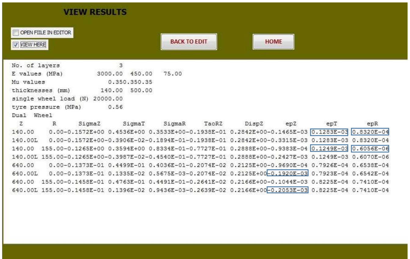
Figure I.3 Abridged screen shot of the output page
