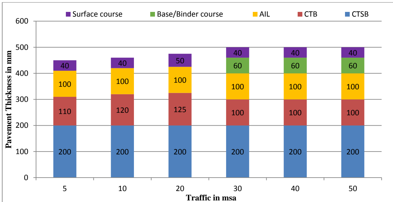
Figure 12.9 Catalogue for pavement with bituminous surface course with CTSB, CTB and granular crack relief layer - Effective CBR 5% (Plate-9)
