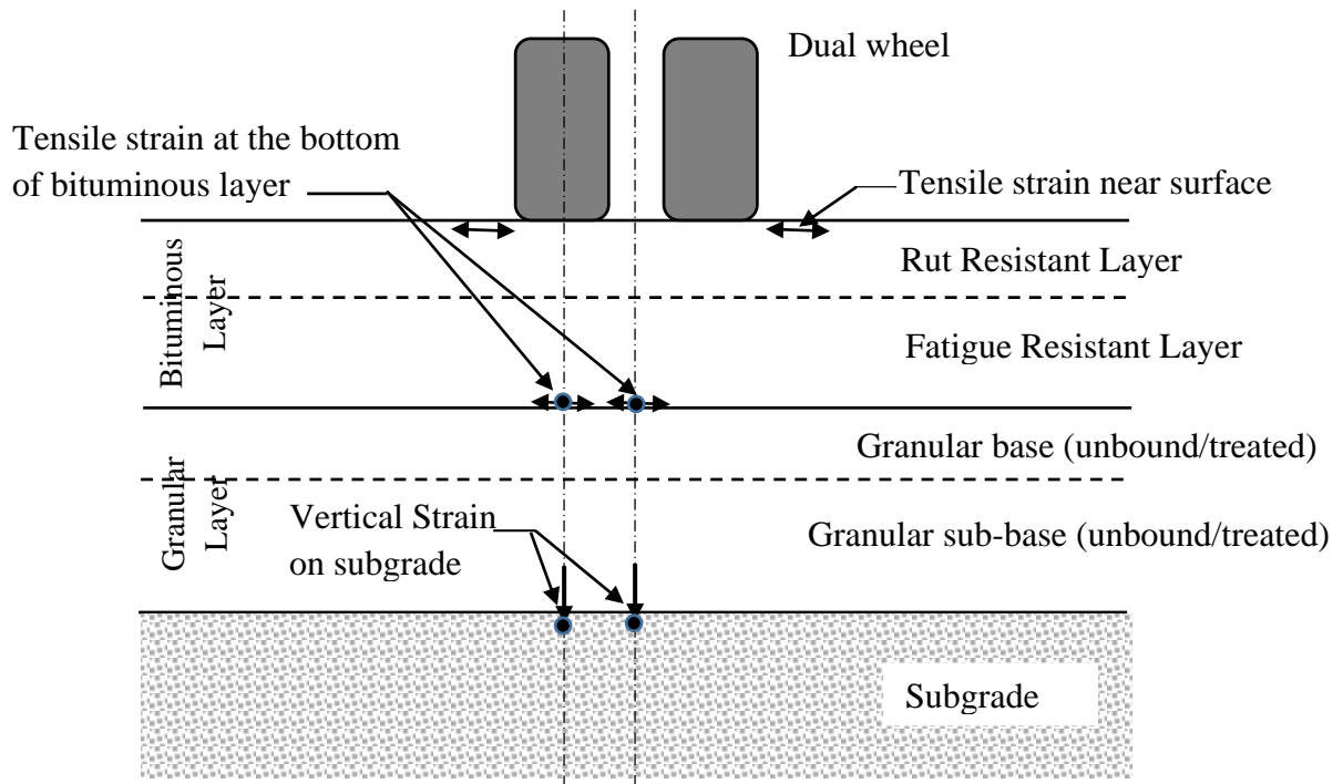
Figure 3.1 A pavement section with bituminous layer(s), granular base and GSB showing the locations of critical strains
