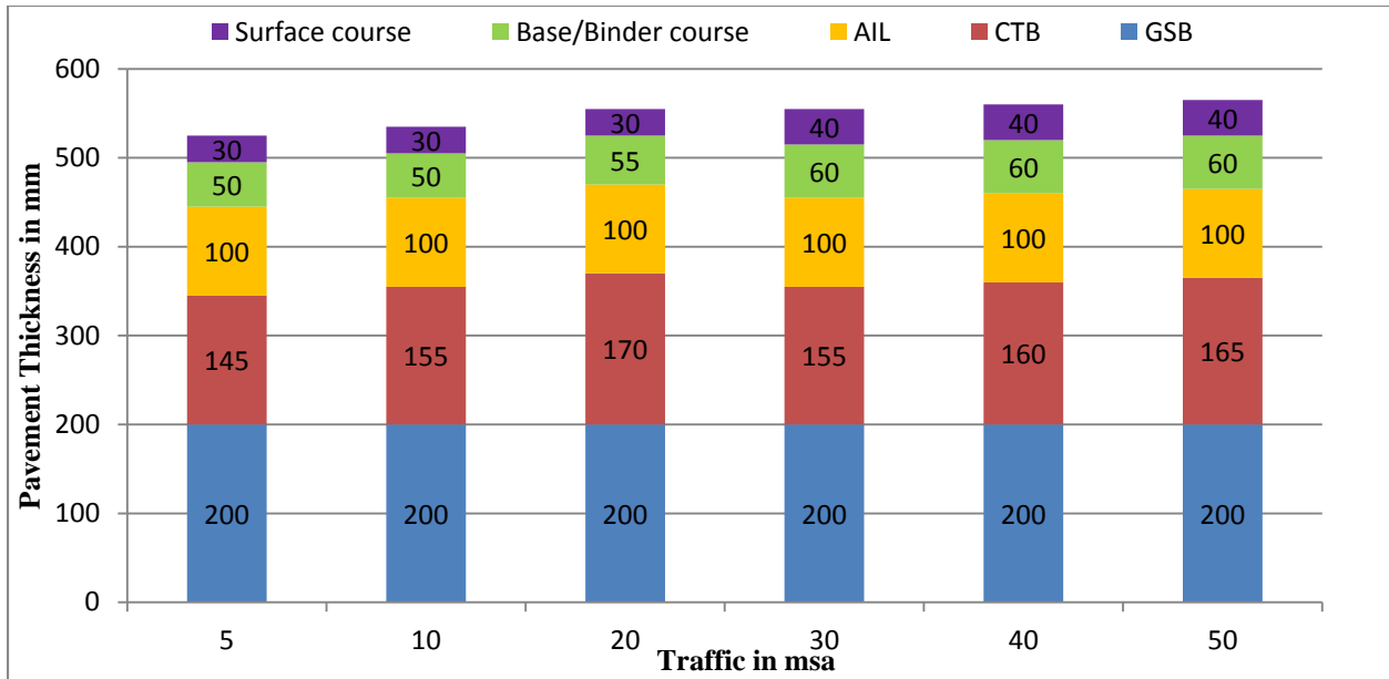
Figure 12.36 Catalogue for pavement with bituminous surface course with GSB, CTB and granular crack relief layer - Effective CBR 8% (Plate-36)
