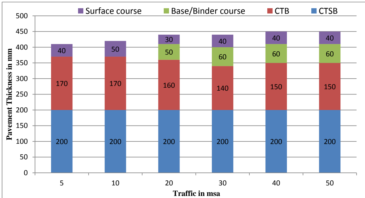
Figure 12.17 Catalogue for pavement with bituminous surface course with CTSB, CTB and SAMI - Effective CBR 5% (Plate-17)
