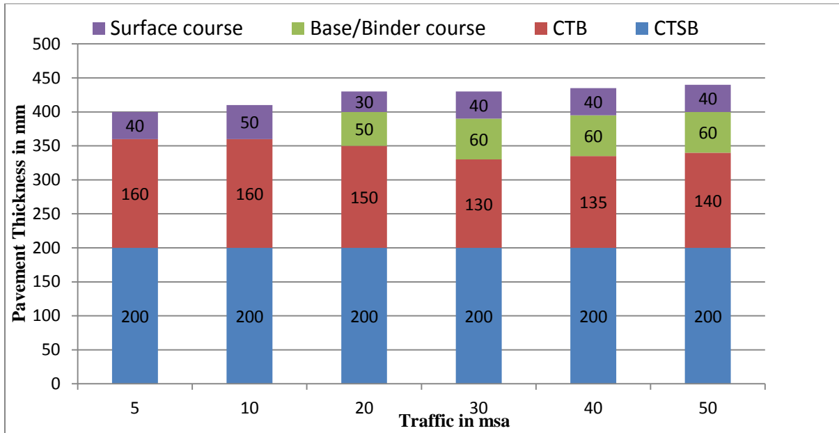
Figure 12.22 Catalogue for pavement with bituminous surface course with CTSB, CTB and SAMI - Effective CBR 10% (Plate-22)
