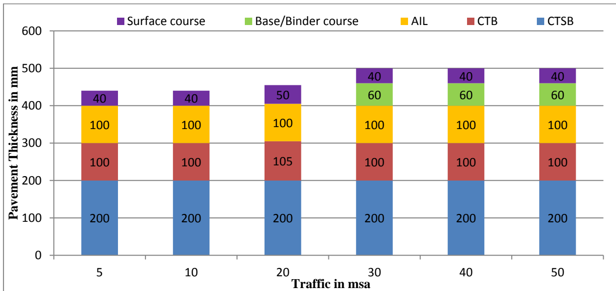
Figure 12.15 Catalogue for pavement with bituminous surface course with CTSB, CTB and granular crack relief layer - Effective CBR 12% (Plate-15)
