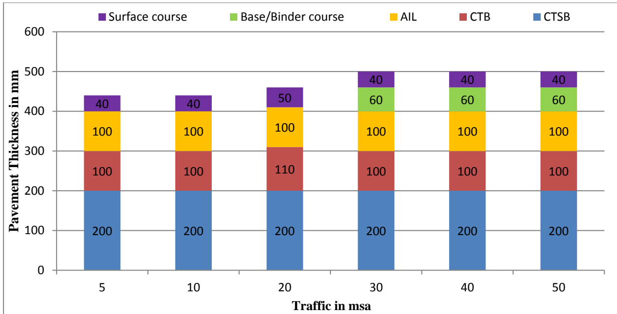
Figure 12.14 Catalogue for pavement with bituminous surface course with CTSB, CTB and granular crack relief layer - Effective CBR 10% (Plate-14)
