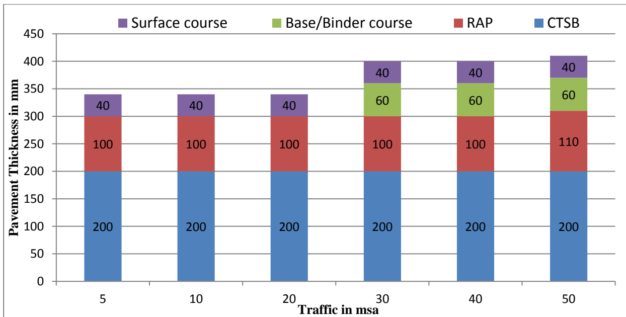
Figure 12.29 Catalogue for pavement with bituminous surface course with CTSB and emulsion/foam bitumen stabilised RAP/virgin aggregate - Effective CBR 9% (Plate-29)
