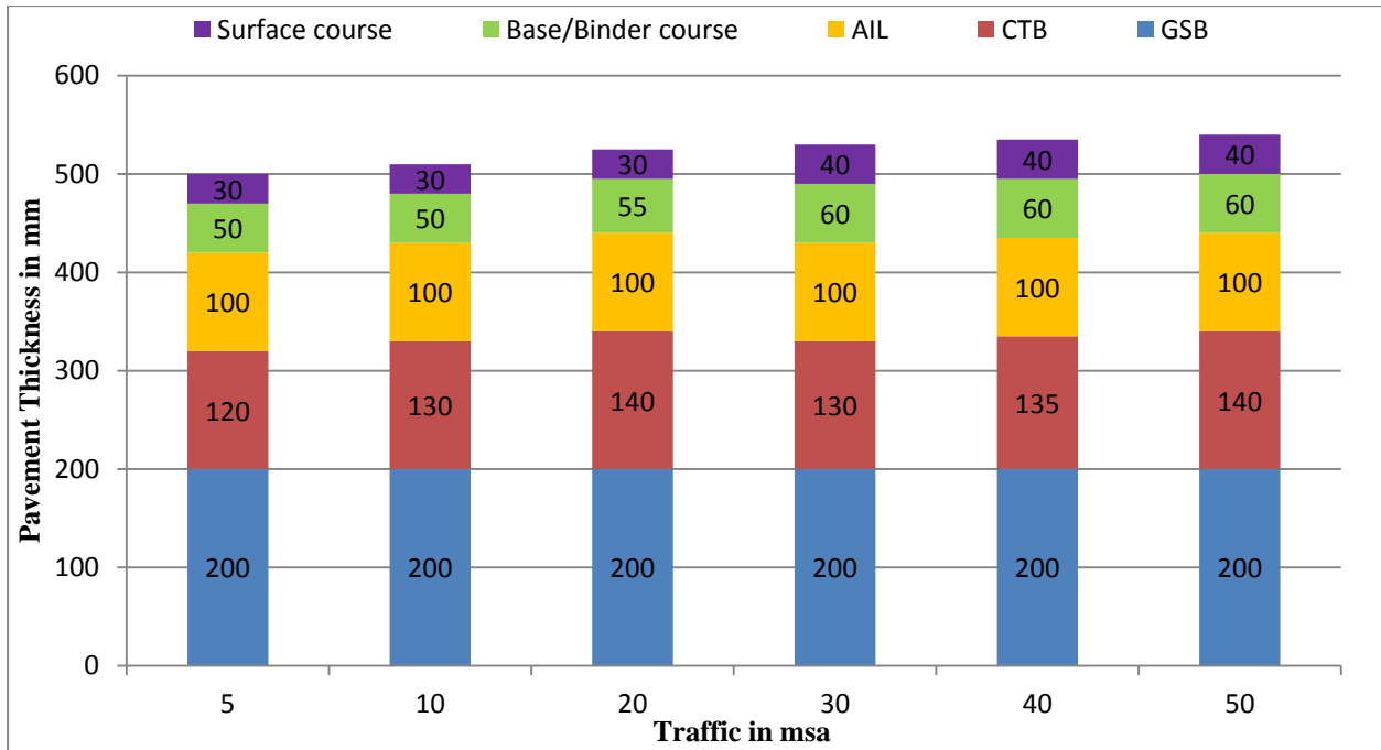
Figure 12.40 Catalogue for pavement with bituminous surface course with GSB, CTB and granular crack relief layer - Effective CBR 15% (Plate-40)
