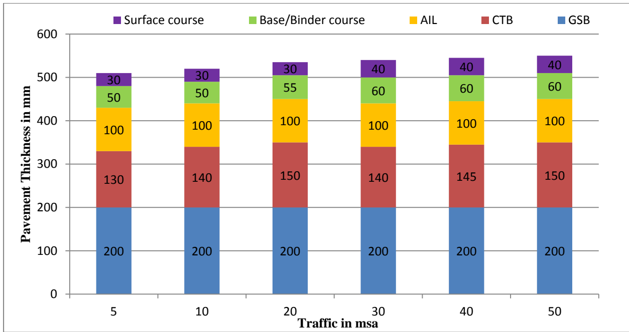
Figure 12.39 Catalogue for pavement with bituminous surface course with GSB, CTB and granular crack relief layer - Effective CBR 12% (Plate-39)
