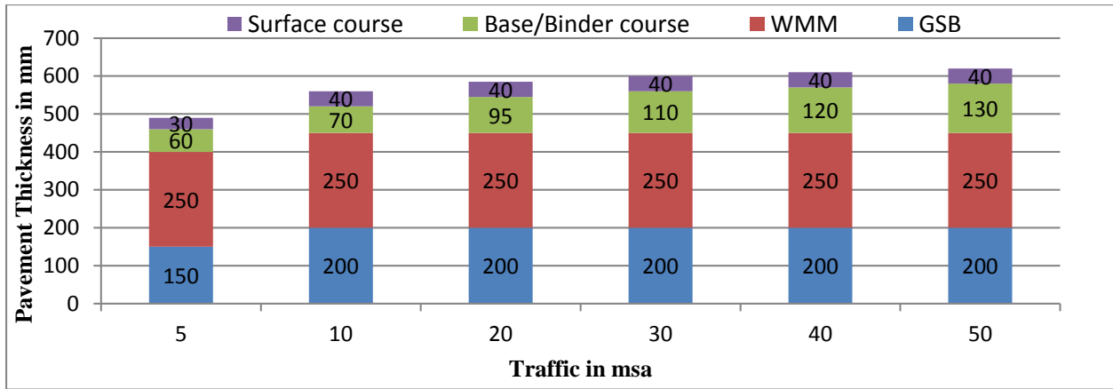
Figure 12.2 Catalogue for pavement with bituminous surface course with granular base and sub-base - Effective CBR 6% (Plate-2)
