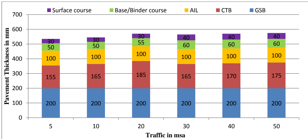
Figure 12.35 Catalogue for pavement with bituminous surface course with GSB, CTB and granular crack relief layer - Effective CBR 7% (Plate-35)
