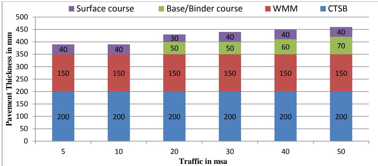
Figure 12.44 Catalogue for pavement with bituminous surface course with CTSB and granular base course - Effective CBR 8% (Plate-44)
