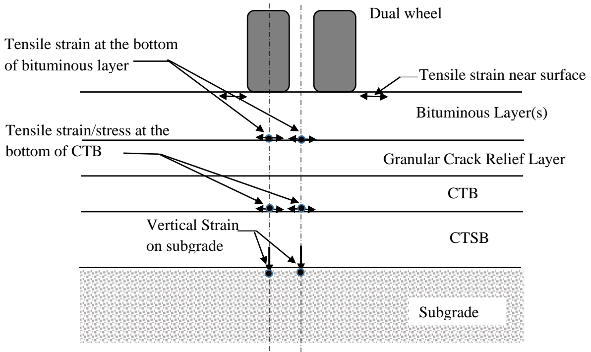
Figure 3.2 A pavement section with bituminous layer(s), granular crack relief layer, CTB, and CTSB showing the locations of critical strains
