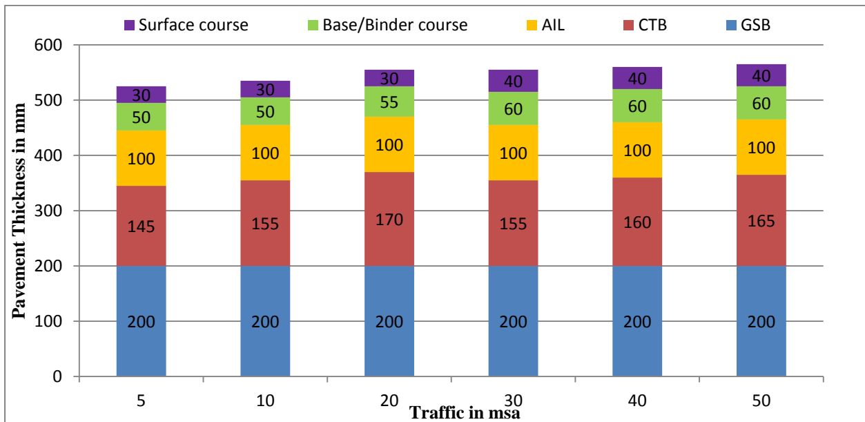
Figure 12.37 Catalogue for pavement with bituminous surface course with GSB, CTB and granular crack relief layer - Effective CBR 9% (Plate-37)
