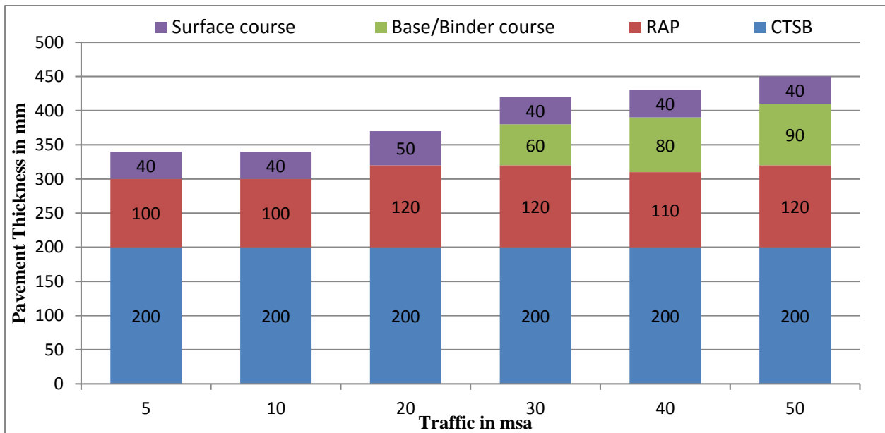
Figure 12.25 Catalogue for pavement with bituminous surface course with CTSB and emulsion/foam bitumen stabilised RAP/virgin aggregate - Effective CBR 5% (Plate-25)
