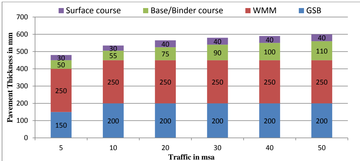
Figure 12.5 Catalogue for pavement with bituminous surface course with granular base and sub-base - Effective CBR 9% (Plate-5)
