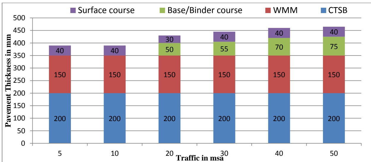
Figure 12.43 Catalogue for pavement with bituminous surface course with CTSB and granular base course - Effective CBR 7% (Plate-43)
