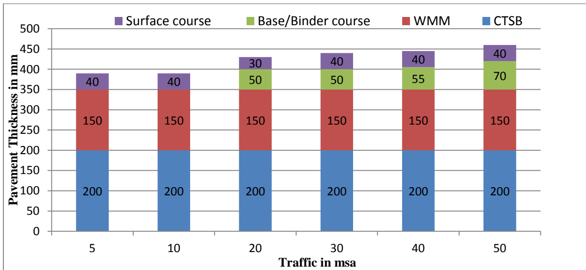
Figure 12.45 Catalogue for pavement with bituminous surface course with CTSB and granular base course - Effective CBR 9% (Plate-45)
