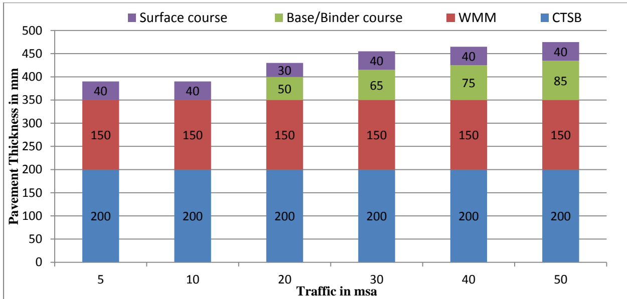
Figure 12.42 Catalogue for pavement with bituminous surface course with CTSB and granular base course - Effective CBR 6% (Plate-42)
