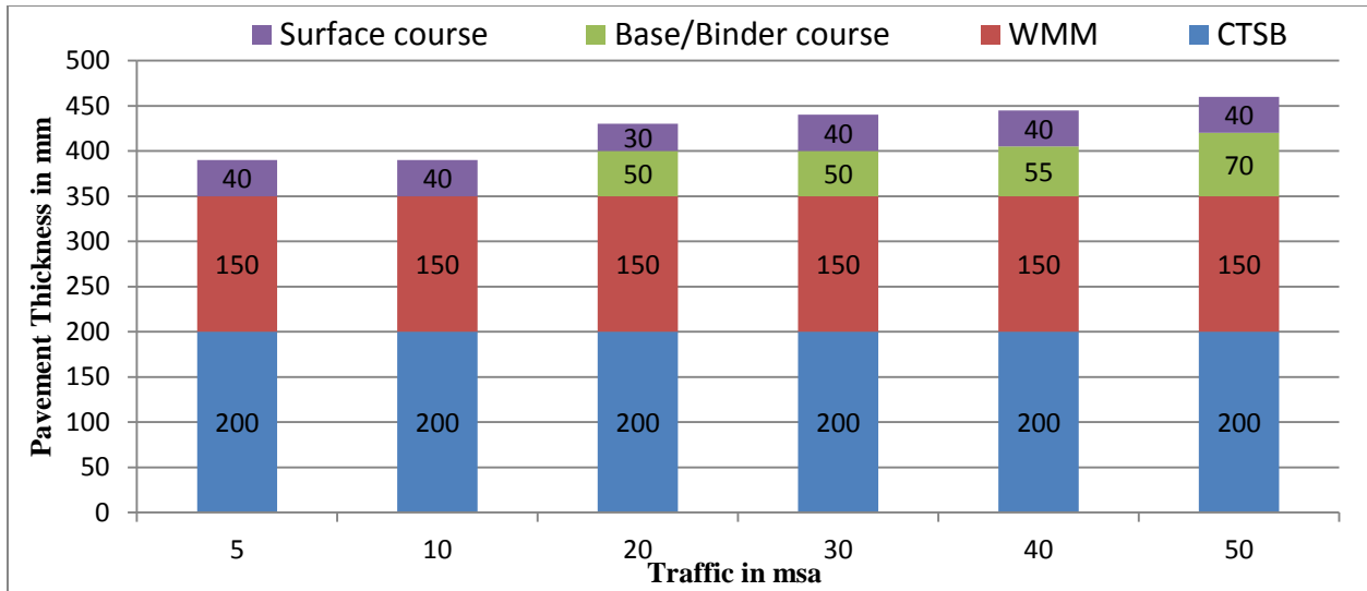
Figure 12.46 Catalogue for pavement with bituminous surface course with CTSB and granular base course - Effective CBR 10% (Plate-46)
