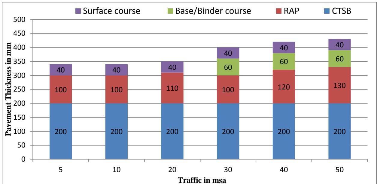
Figure 12.27 Catalogue for pavement with bituminous surface course with CTSB and emulsion/foam bitumen stabilised RAP/virgin aggregate - Effective CBR 7% (Plate-27)
