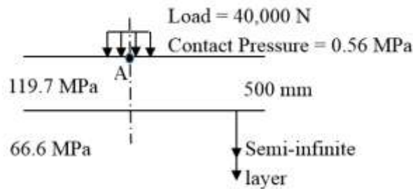
Figure II.1 Two-layer pavement system with subgrade and embankment
