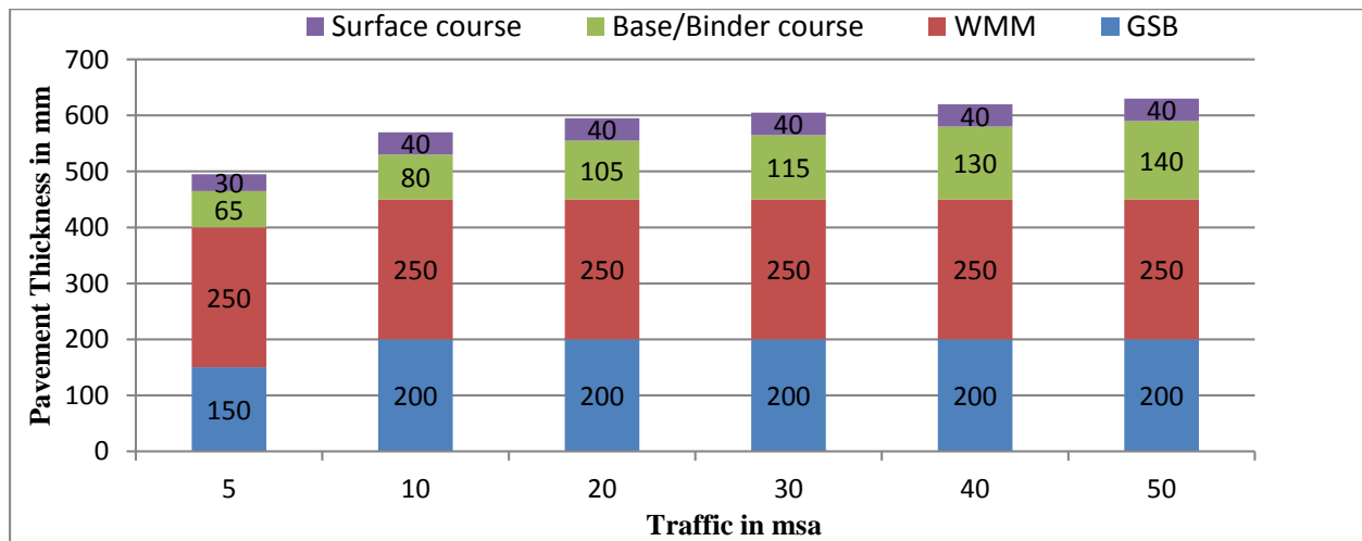
Figure 12.1 Catalogue for pavement with bituminous surface course with granular base and sub-base - Effective CBR 5% (Plate-1)
