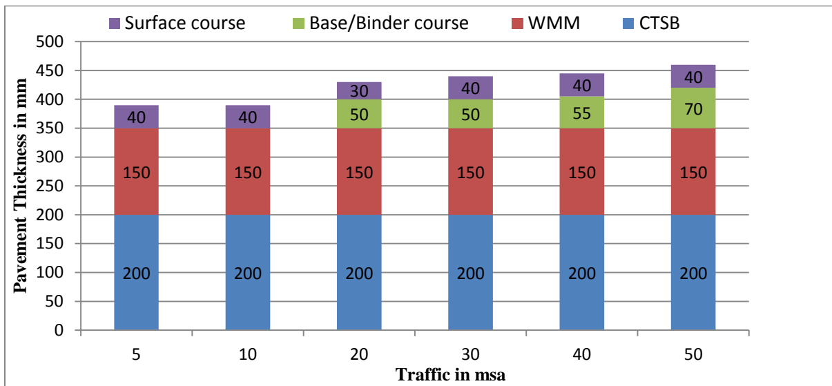
Figure 12.47 Catalogue for pavement with bituminous surface course with CTSB and granular base course - Effective CBR 12% (Plate-47)
