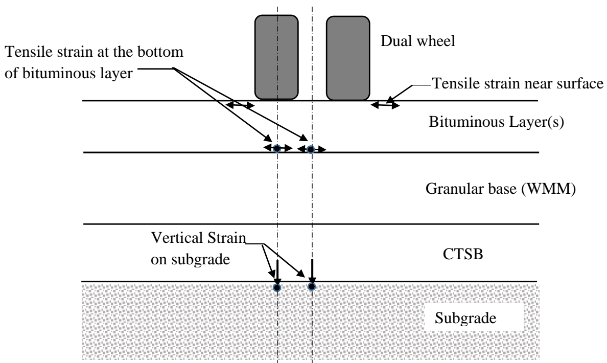
Figure 3.6 A pavement section with bituminous layer(s), granular base (WMM) and CTSB showing the locations of critical strains
