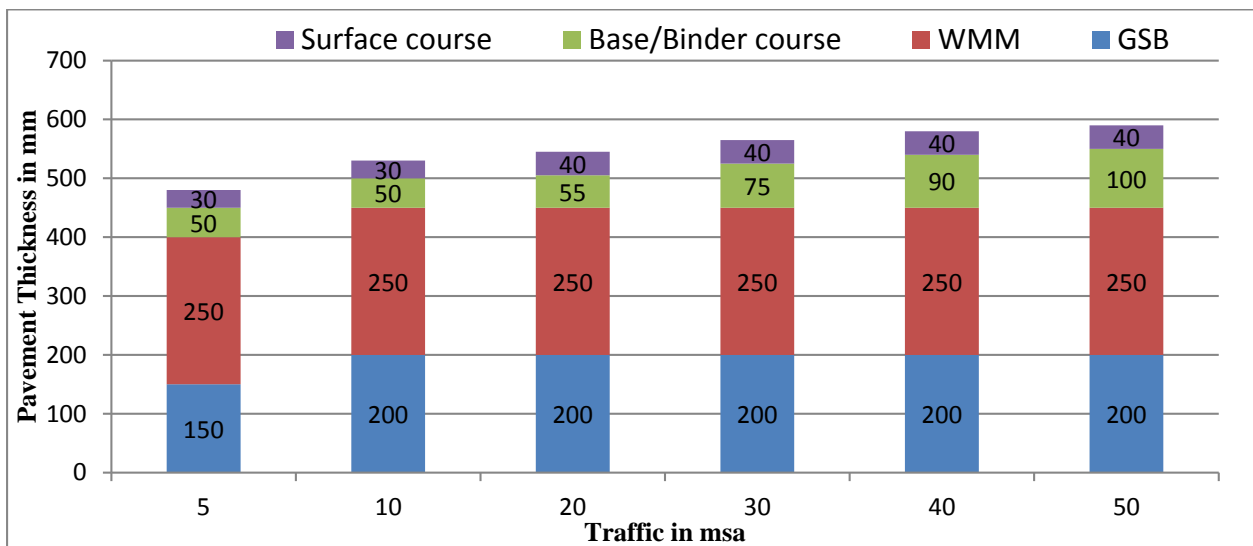
Figure 12.7 Catalogue for pavement with bituminous surface course with granular base and sub-base - Effective CBR 12% (Plate-7)
