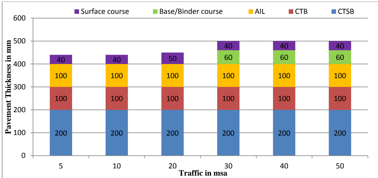
Figure 12.16 Catalogue for pavement with bituminous surface course with CTSB, CTB and granular crack relief layer - Effective CBR 15% (Plate-16)
