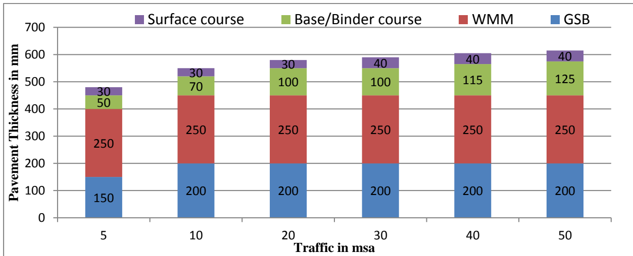
Figure 12.3 Catalogue for pavement with bituminous surface course with granular base and sub-base - Effective CBR 7% (Plate-3)
