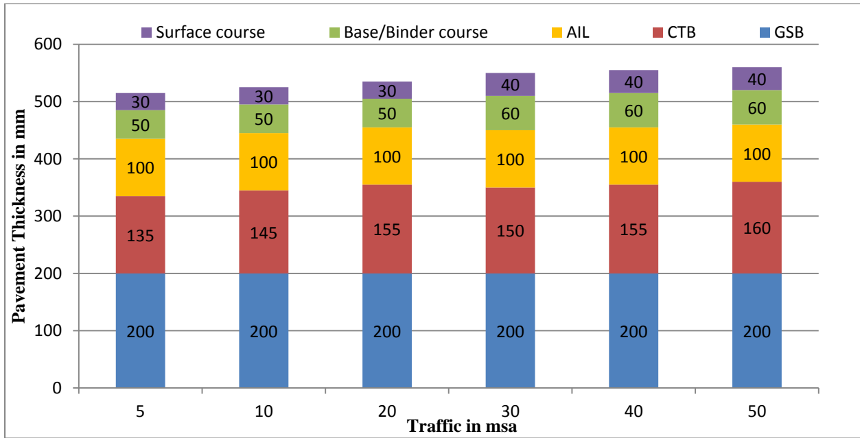
Figure 12.38 Catalogue for pavement with bituminous surface course with GSB, CTB and granular crack relief layer - Effective CBR 10% (Plate-38)
