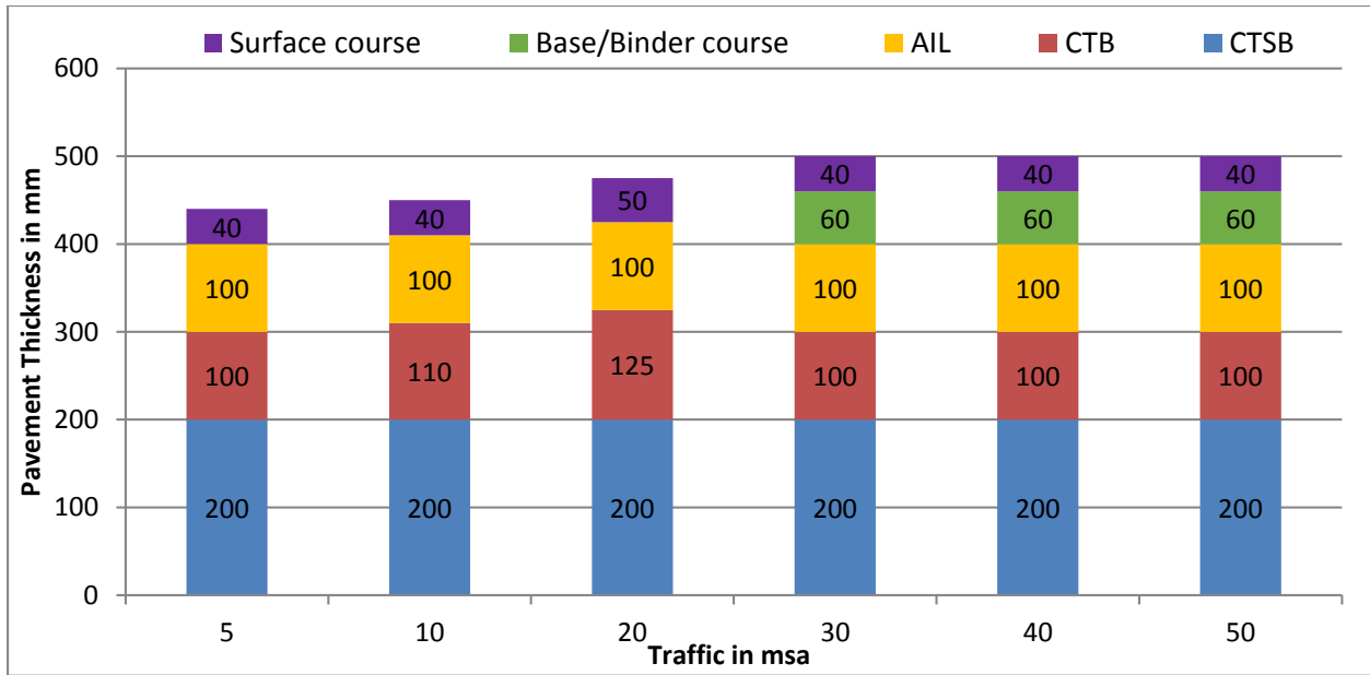
Figure 12.10 Catalogue for pavement with bituminous surface course with CTSB, CTB and granular crack relief layer - Effective CBR 6% (Plate-10)
