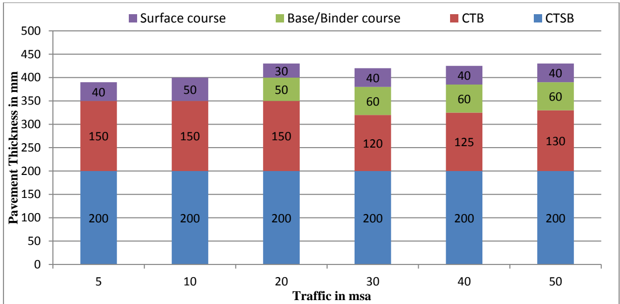
Figure 12.24 Catalogue for pavement with bituminous surface course with CTSB, CTB and SAMI - Effective CBR 15% (Plate-24)
