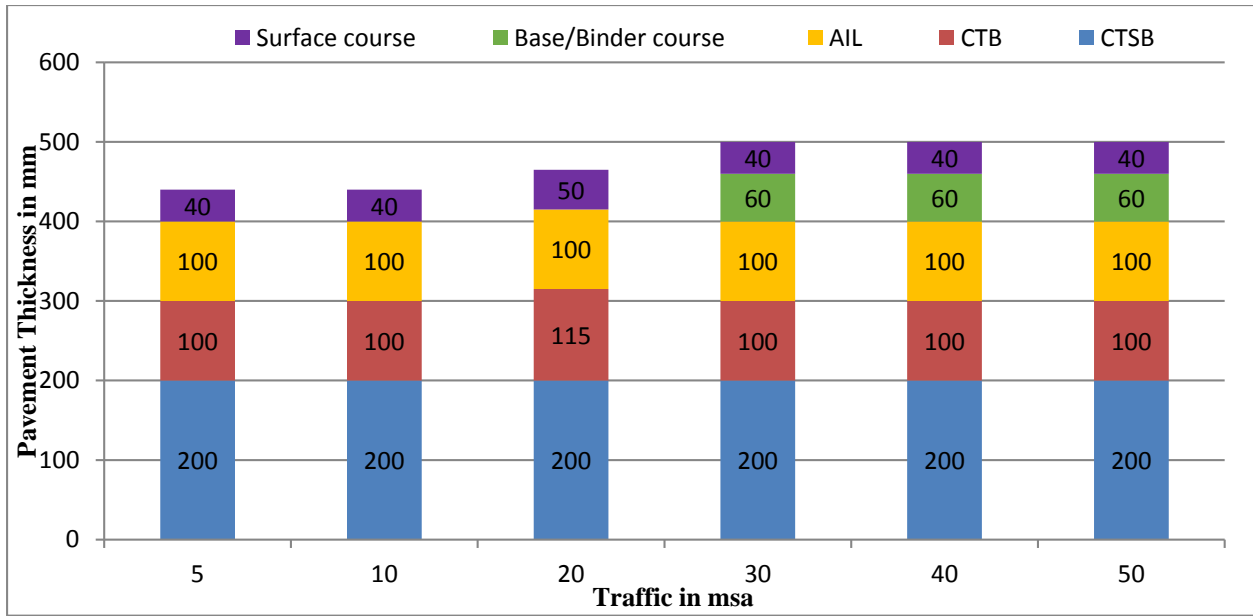
Figure 12.12 Catalogue for pavement with bituminous surface course with CTSB, CTB and granular crack relief layer - Effective CBR 8% (Plate-12)
