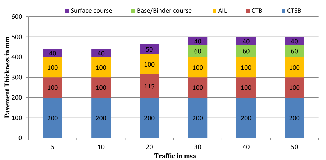
Figure 12.13 Catalogue for pavement with bituminous surface course with CTSB, CTB and granular crack relief layer - Effective CBR 9% (Plate-13)
