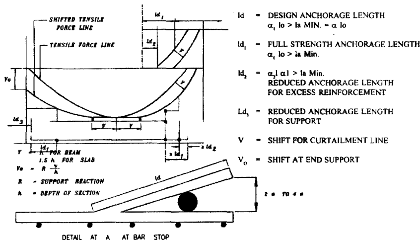
Fig. 4. Curtailment and anchorage of bars in tension zone
