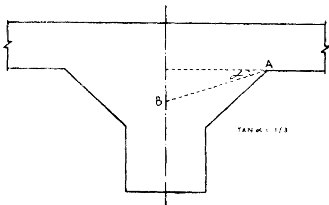
Fig. 9. Portion below line AB to be ignored for effective depth
