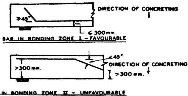
Fig. 1. Bonding zones
