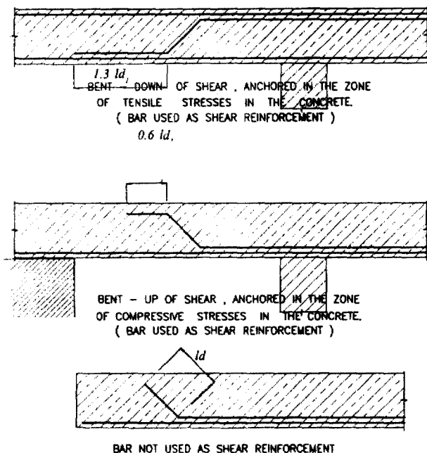
Fig. 5. Anchorage of bars bent up (down)
