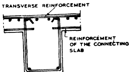
CLOSING WITH T-BEAMS IN THE AREA OF THE SLAB BOTH FOR COMPRESSION AND TENSION ZONE
