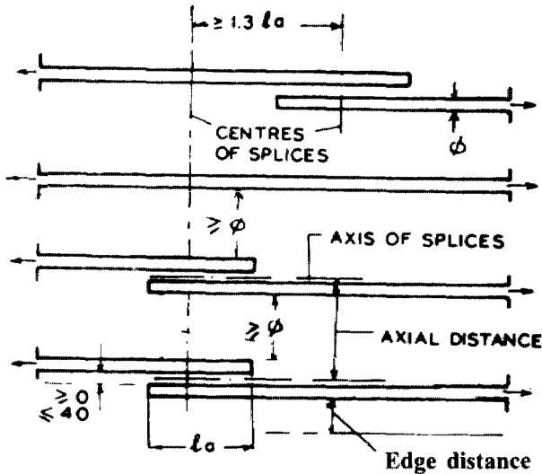
Fig. 7. Longitudinal staggering and transverse distance of reinforcing bars in the region of lap splices (dimensions in mm)
