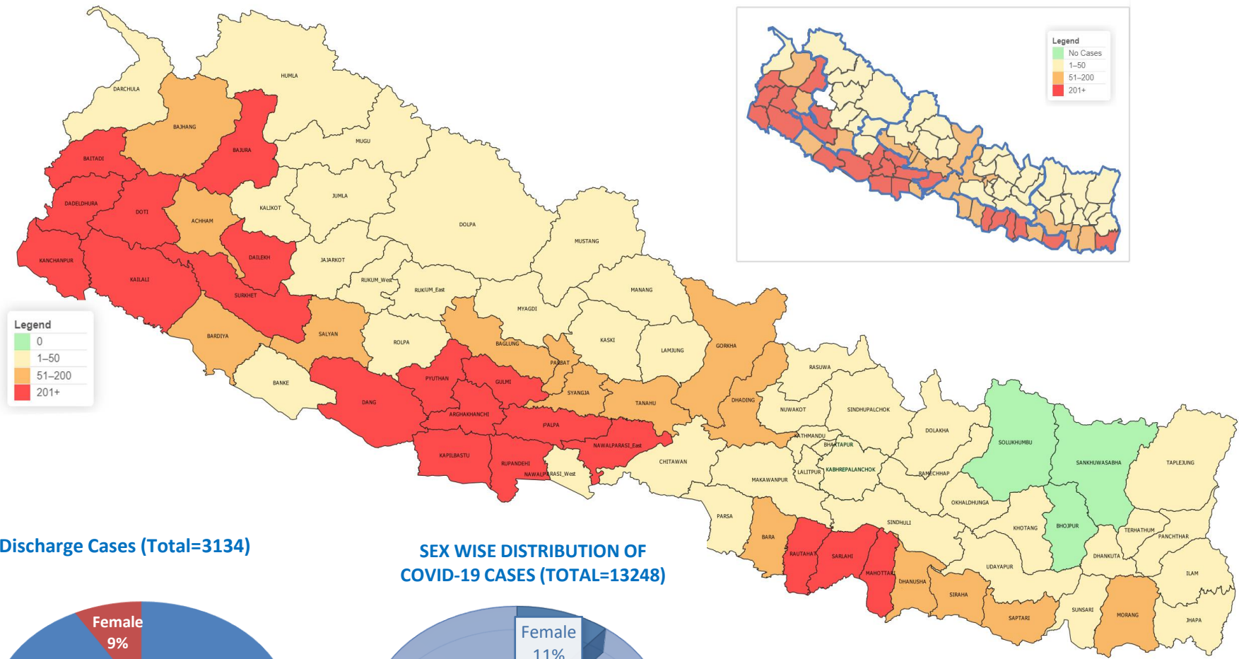
Cumulative Cases
