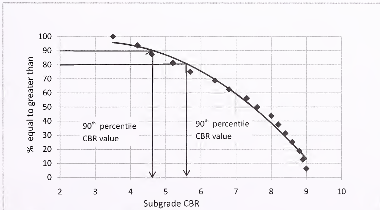
Fig. IV.1 Evaluation of Subgrade CBR for Pavement Design
