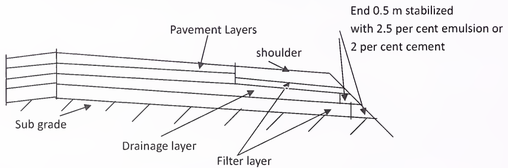
Fig. 11.2 Pavement with Filter and Drainage Layers
