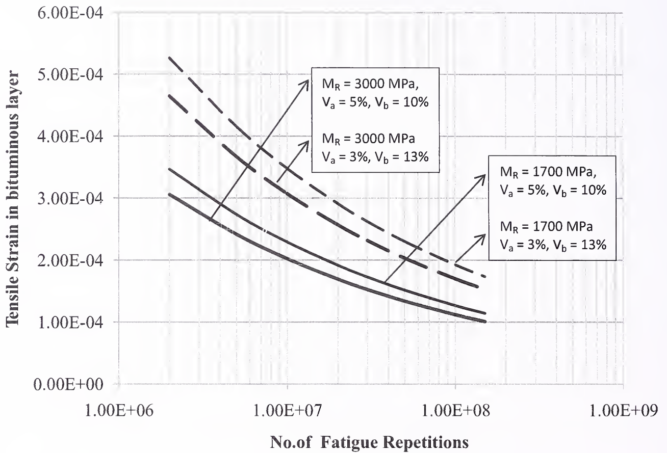
Fig. I-2 Effect of Air Void and Volume of Bitumen on Fatigue Life Bituminous Layer
