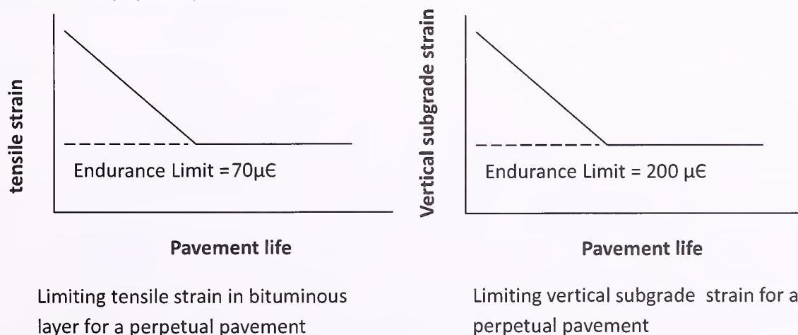
Fig. II-1 Limiting Design Strain for a Perpetual Pavement
