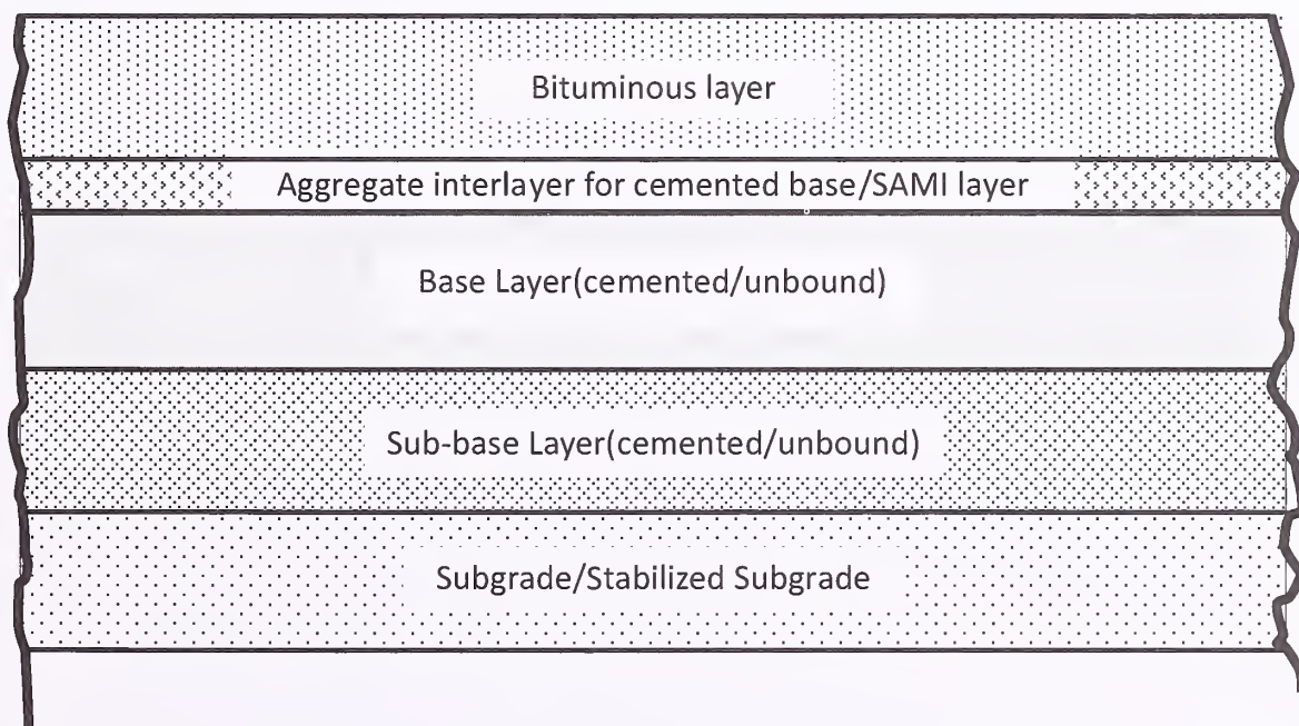
Fig. 7.1 Different Layers of Bituminous Pavement
