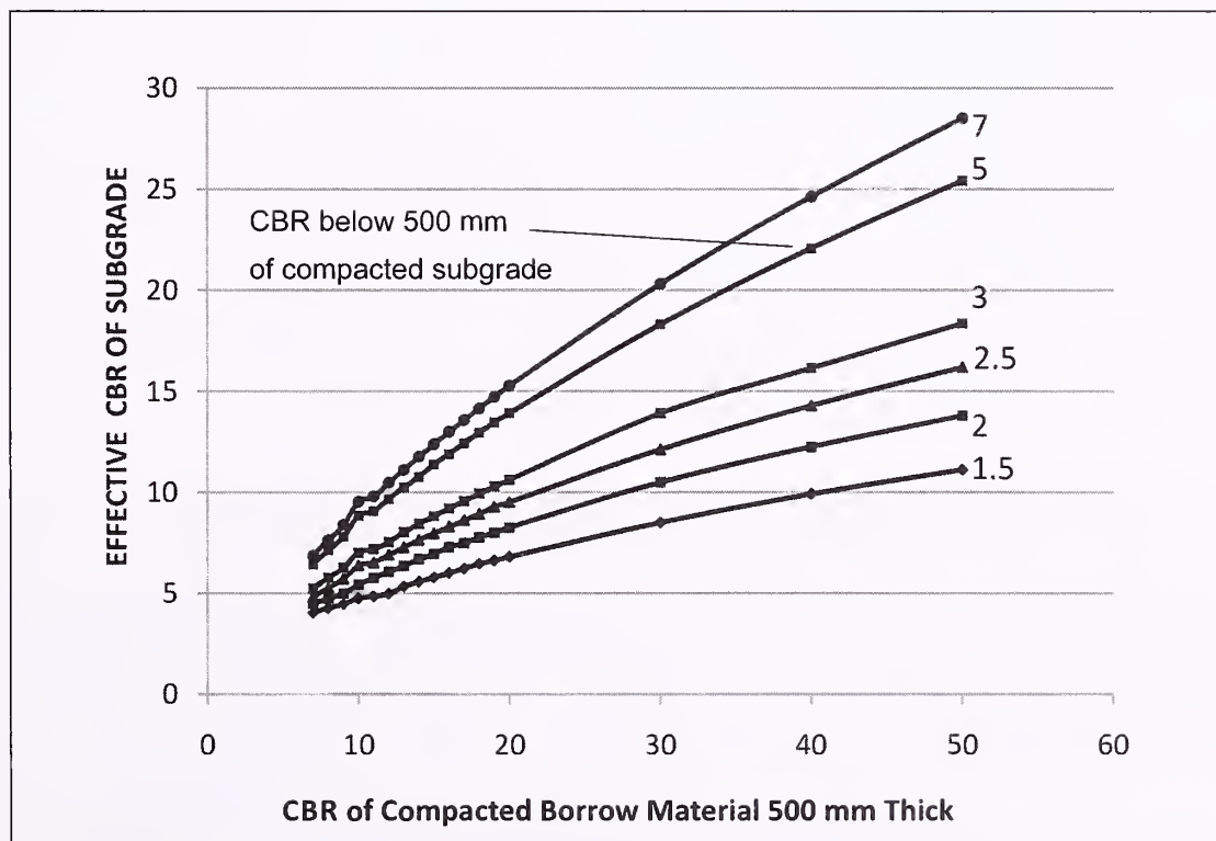
Fig. 5.1 Effective CBR of Subgrade
