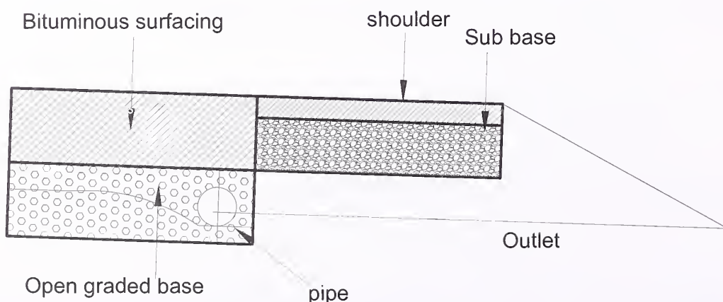
Fig. 11.3 Longitudinal Pipe at the Edge of the Drainage Layer with Outlet Pipe
