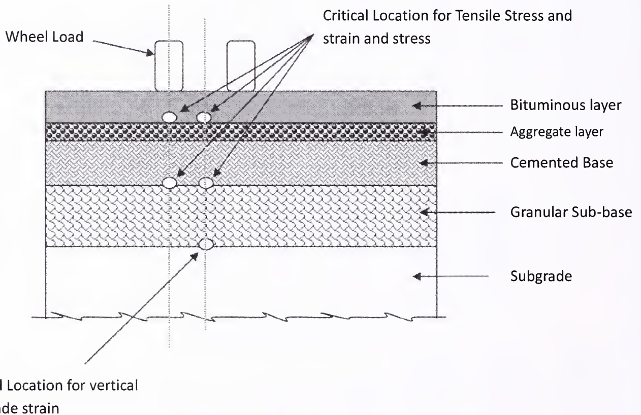
Fig. 10.5 Bituminous Surfacing, Cement Treated Base and Granular Sub-base with Aggregate Interlayer
