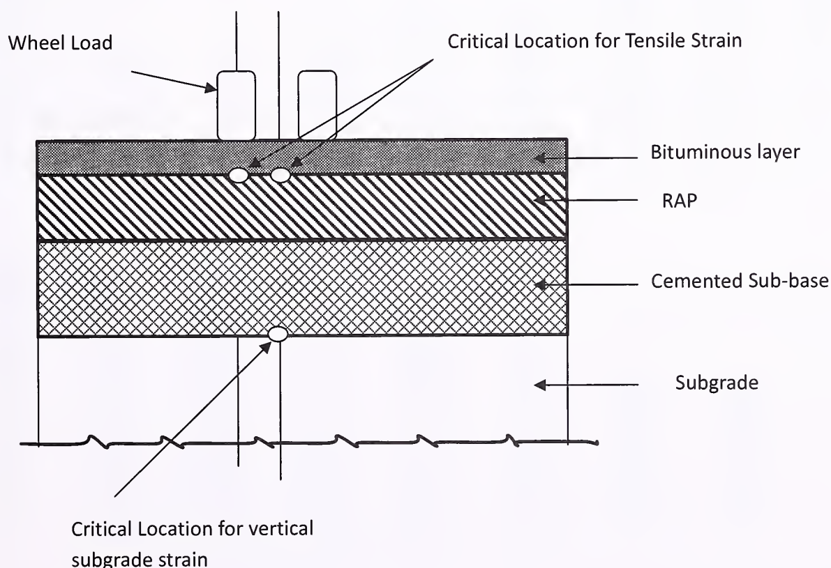
Fig. 10.4 Bituminous Surfacing with RAP and Cemented Sub-base
