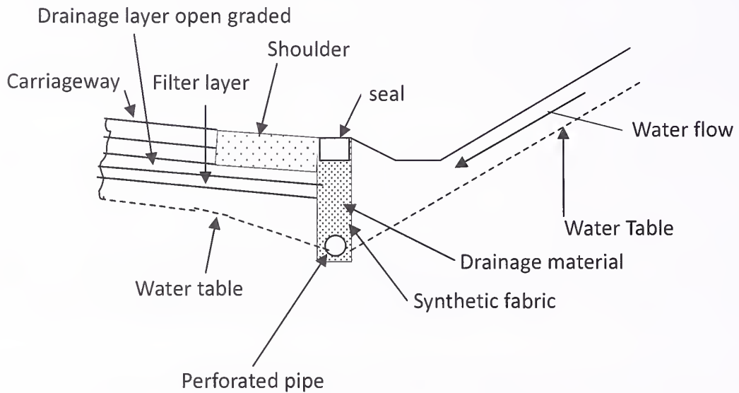
Fig. 11.1 Pavement along a Slope
