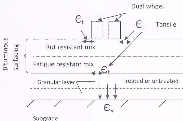
Fig. 6.1 Different Layers of a Flexible Pavement
