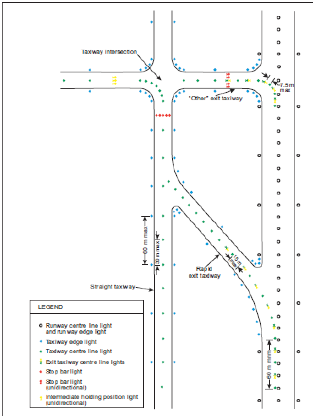
Figure 5-26. Taxiway lighting
