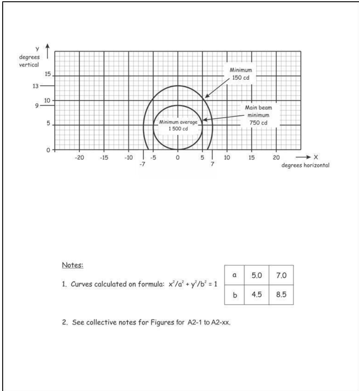
Figure A2-26. Isocandela diagram for take-off and hold lights (THL) (red light)
