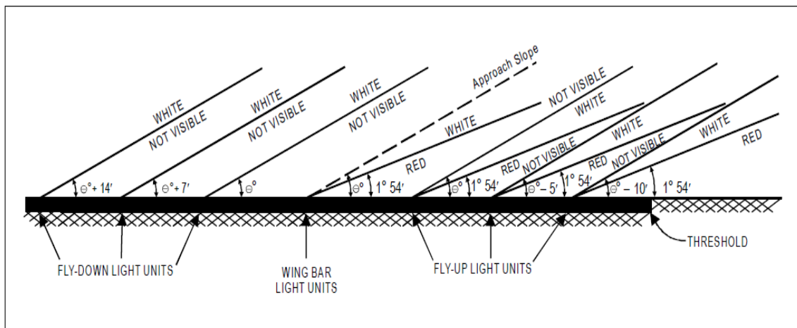
Figure 5-18. Light beams and elevation settings of T-VASIS and AT-VASIS
