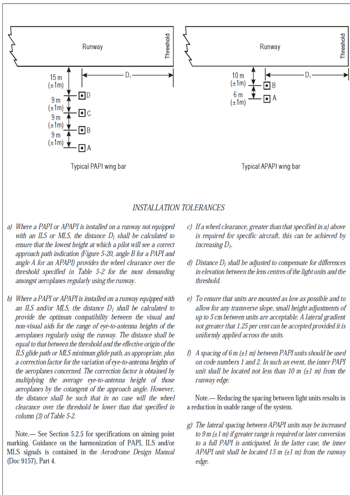
Figure 5-19. Siting of PAPI and APAPI
