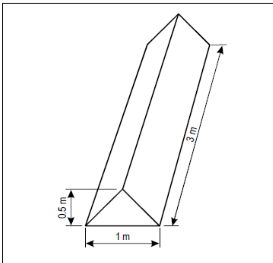
Figure 5-34. Boundary markers
