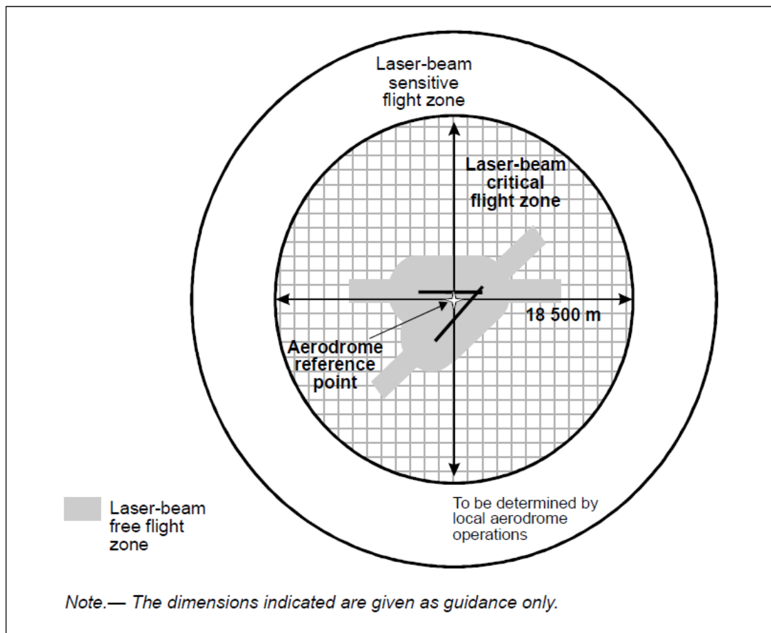
Figure 5-11. Protection flight zones
