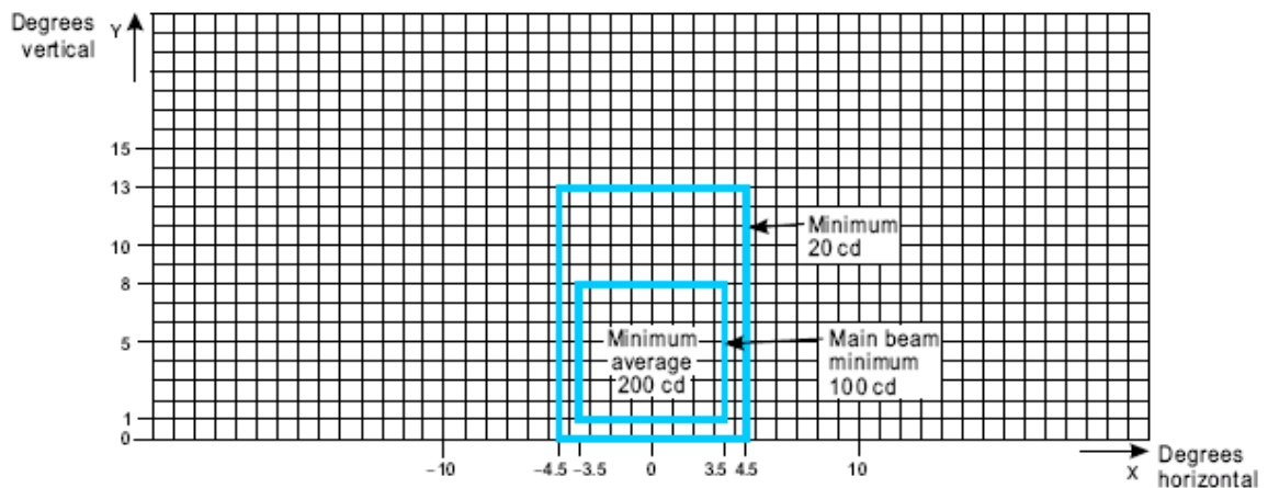
Figure A2-12. Isocandela diagram for taxiway centre line (15 m spacing), RELS, no-entry bar and stop bar lights in straight sections intended for use in runway visual range conditions of less than a value of 350 m where large offsets can occur and for low-intensity runway guard lights, Configuration B
