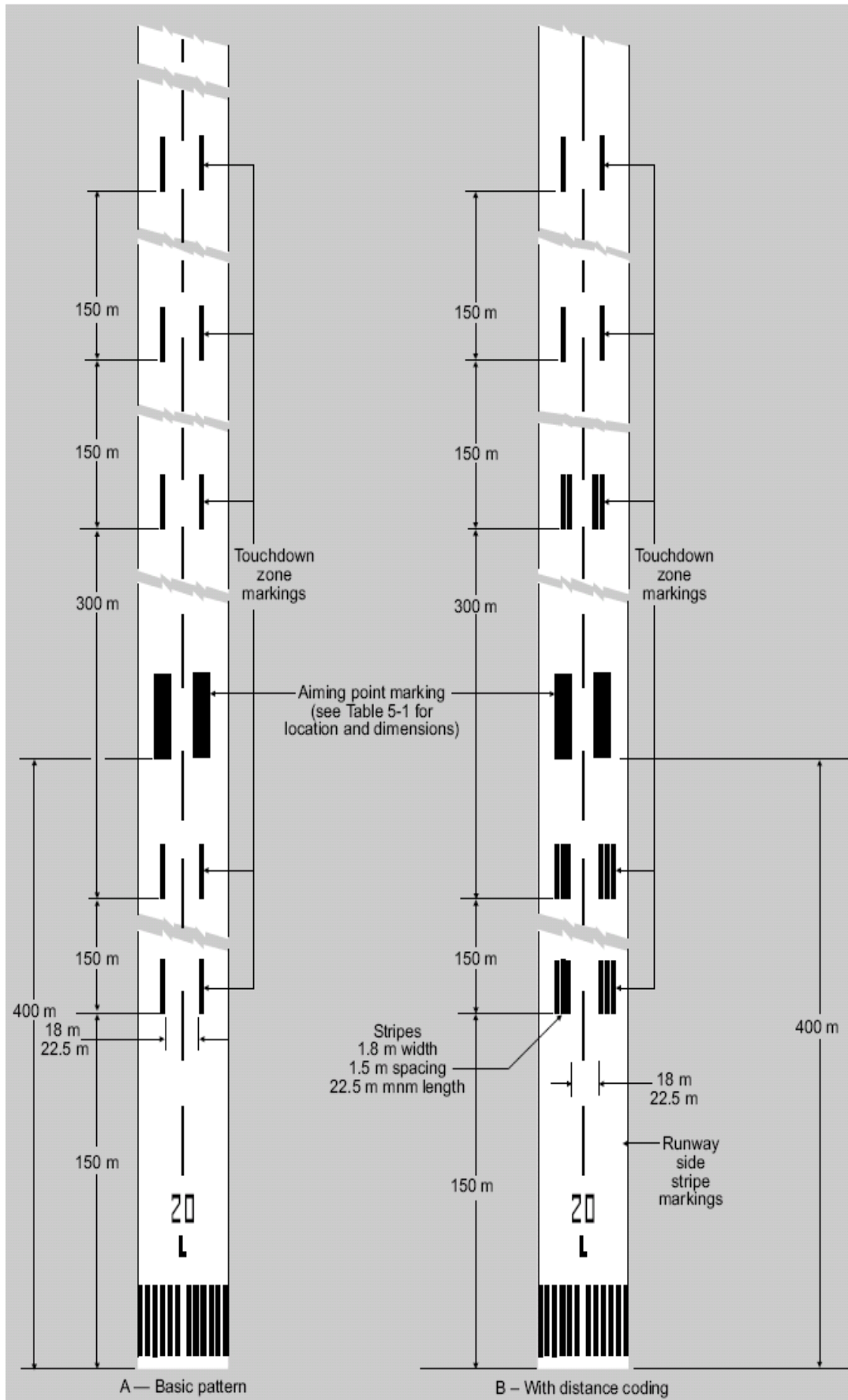
Figure 5-5. Aiming point and touchdown zone markings
