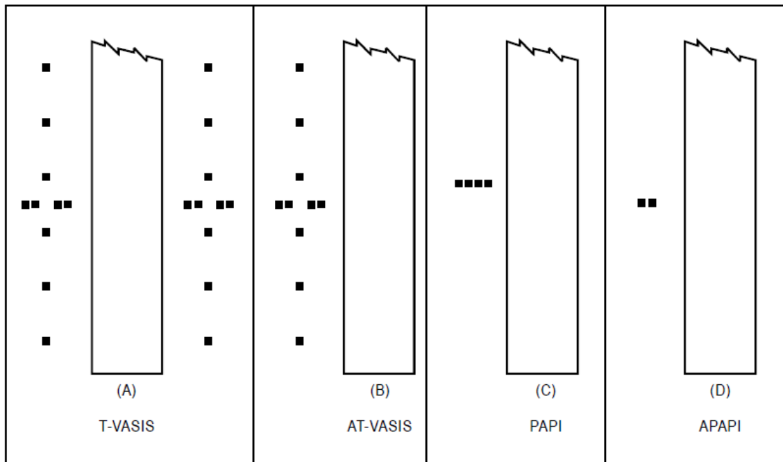
Figure 5-16. Visual approach slope indicator systems
