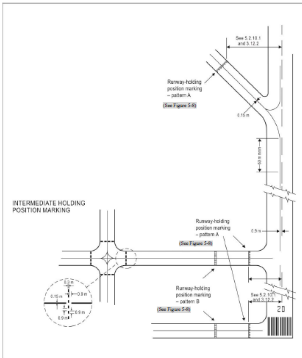
Figure 5-6. Taxiway markings
