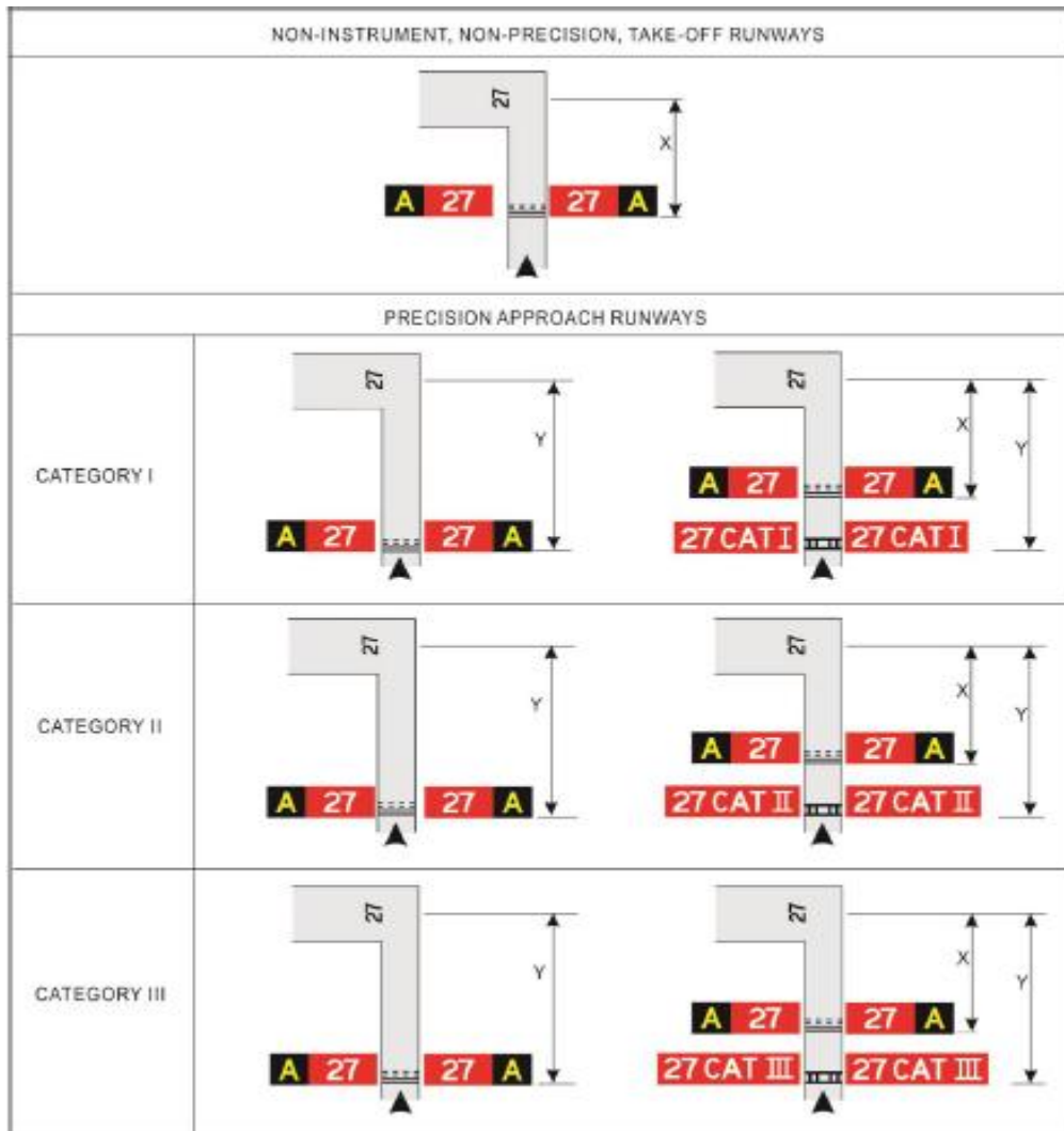
Figure 5-32. Examples of sign positions at taxiway/runway intersections
