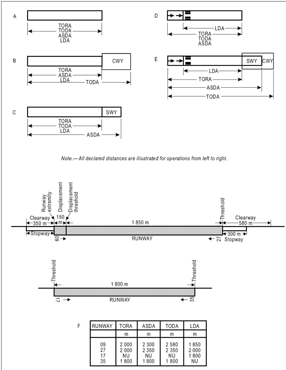
Figure A-1. Illustration of declared distances
