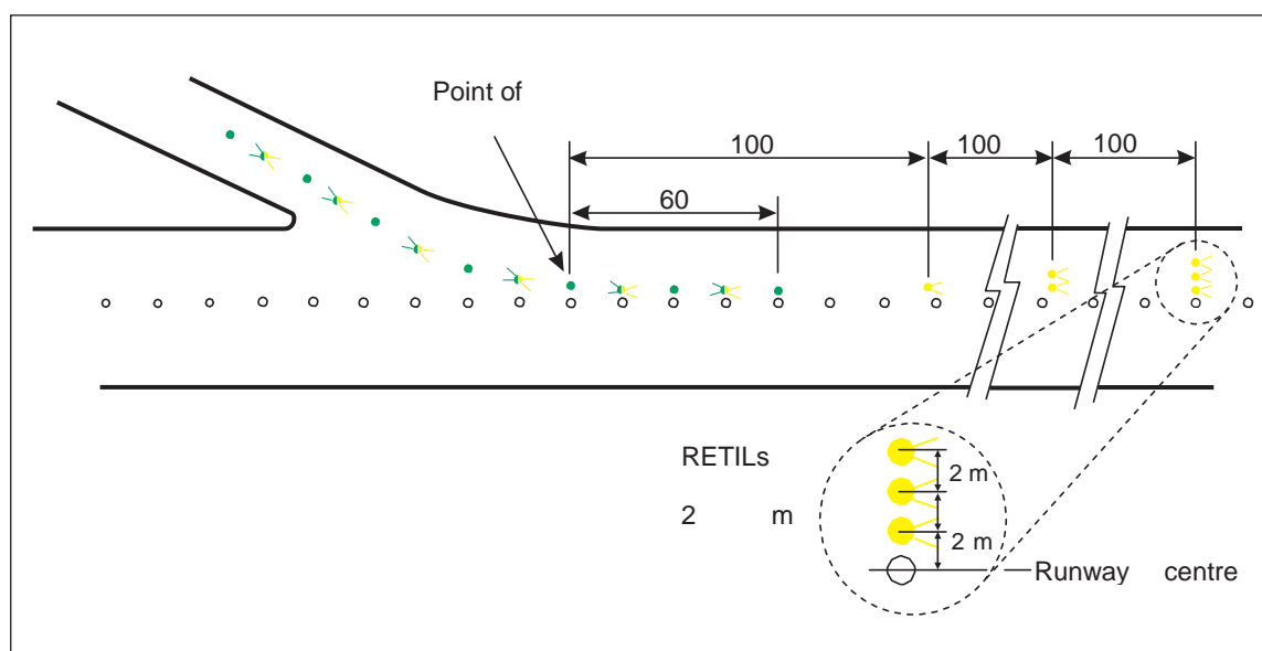
Figure 5-25. Rapid exit taxiway indicator lights (RETILs)
