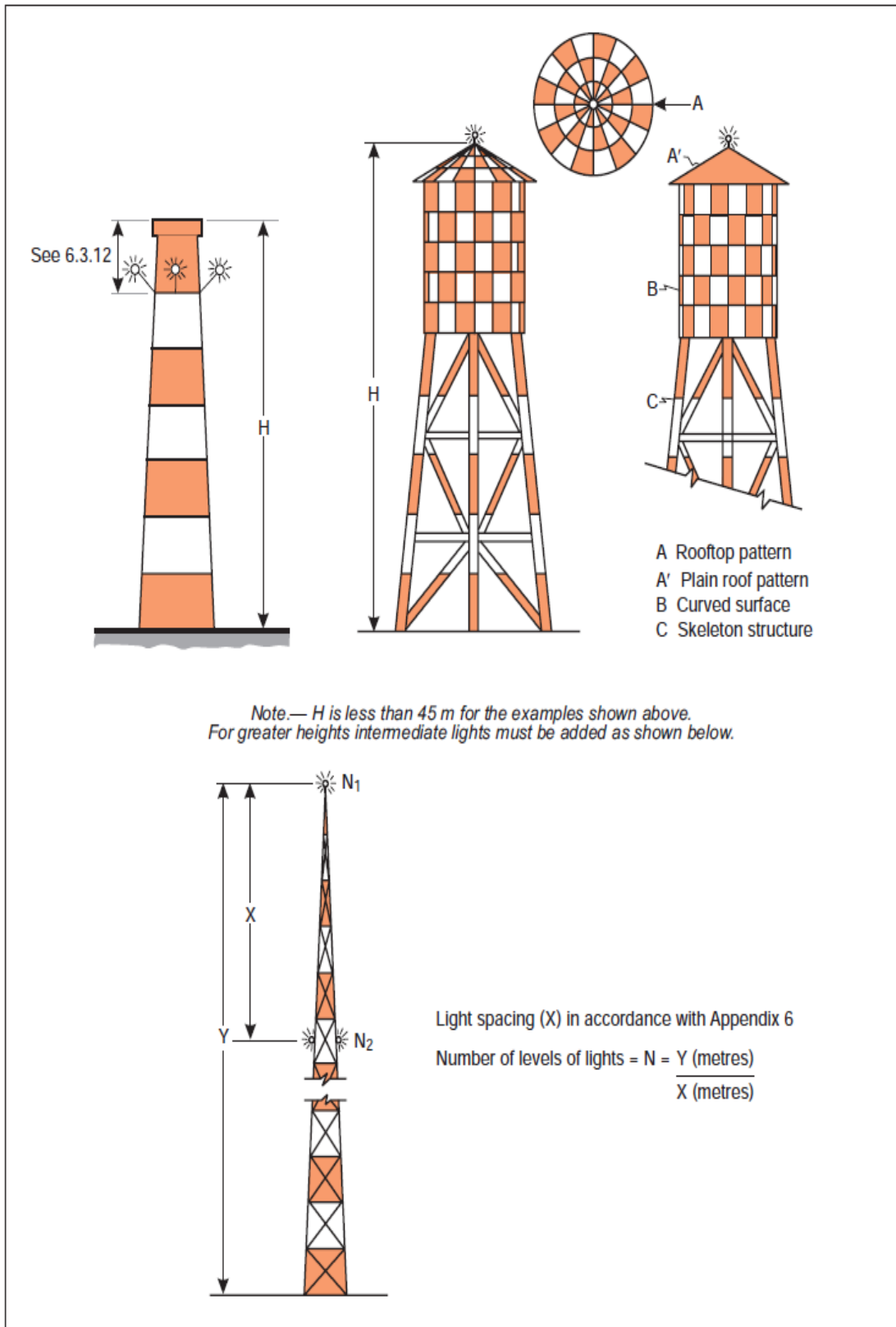
Figure 6-2. Examples of marking and lighting of tall structures
