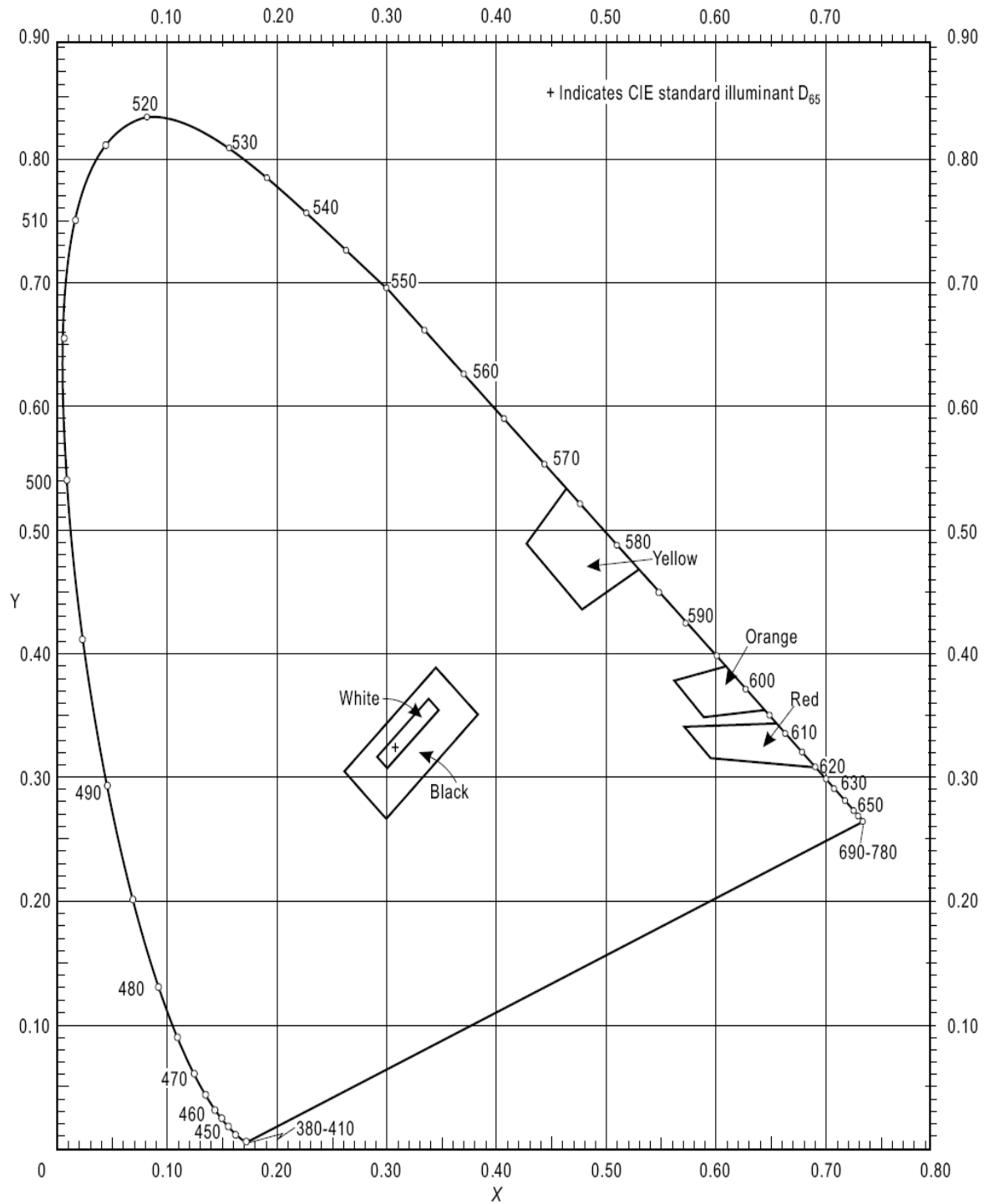
Figure A1-2. Ordinary colours for markings and externally illuminated sign and panels
