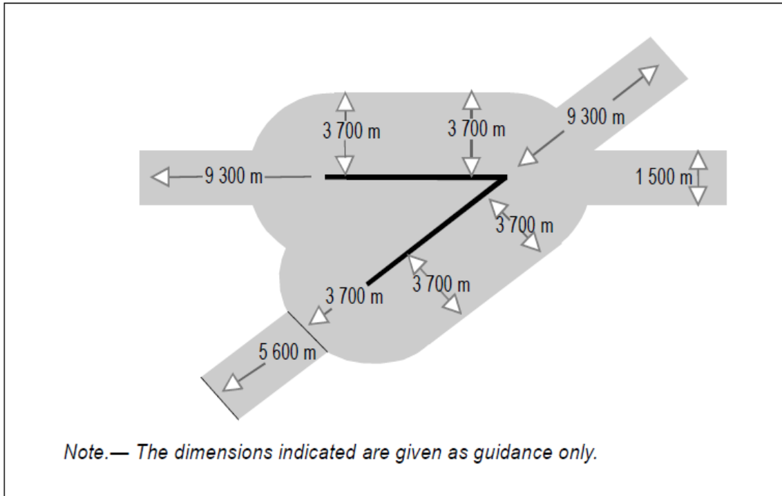
Figure 5-12. Multiple runway laser-beam free flight zone
