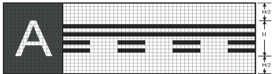
Runway vacated sign (with typical location sign)
