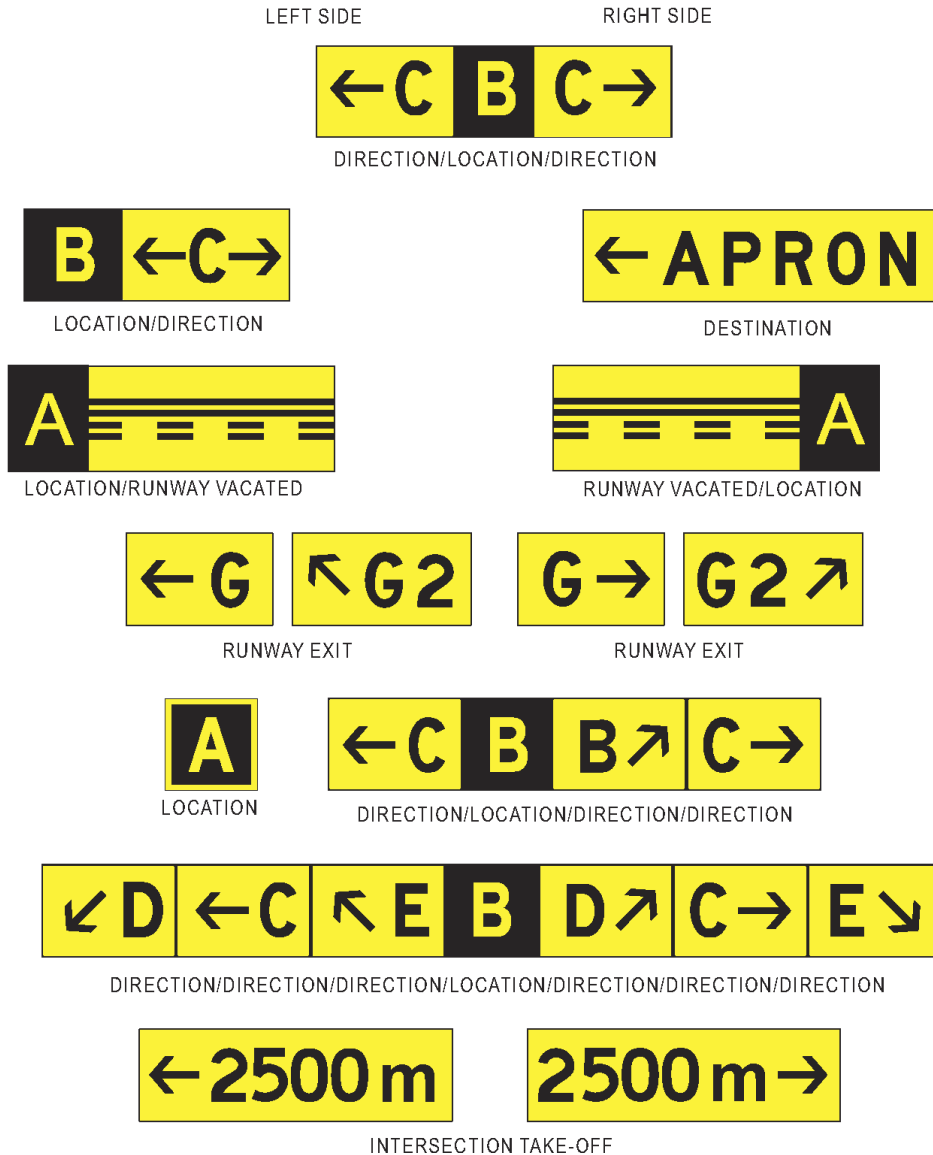
Figure 5-31. Information signs
