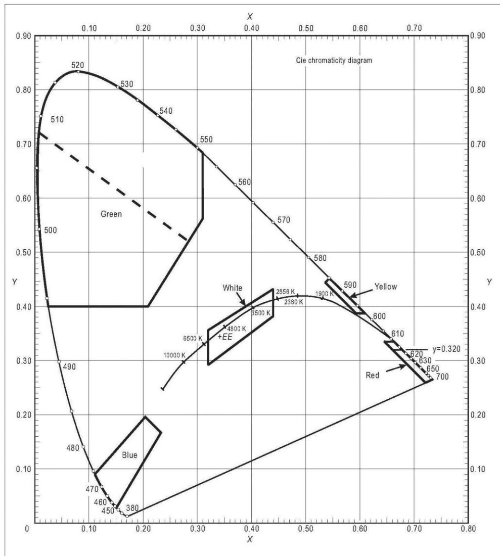
3. Figure A1-1b. Colours for aeronautical ground lights (solid state lighting)
