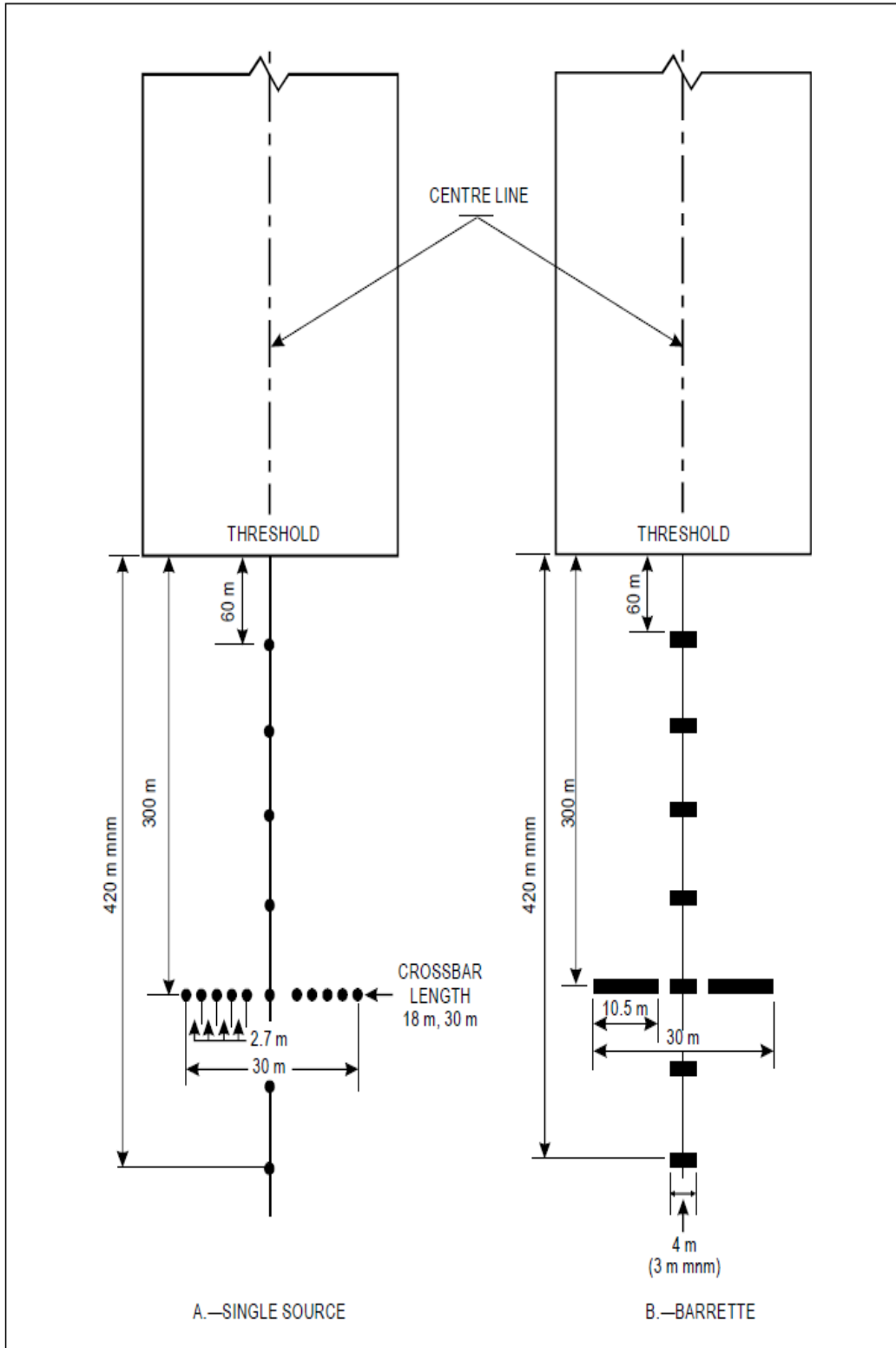
Figure A-7. Simple approach lighting systems
