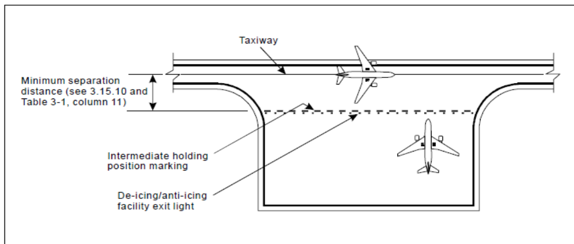
Figure 5-28. Typical remote de-icing/anti-icing facility
