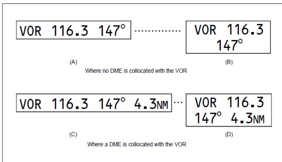
Figure 5-33. VOR aerodrome checkpoint sign
