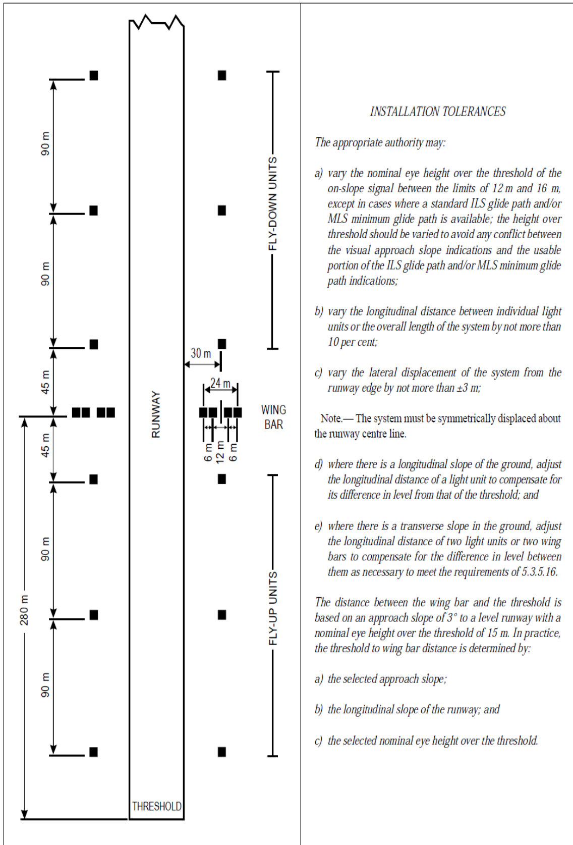
Figure 5-17. Siting of light units for T-VASIS
