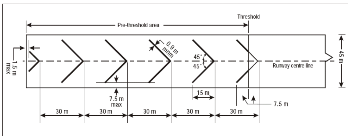
Figure 7-2. Pre-threshold marking
