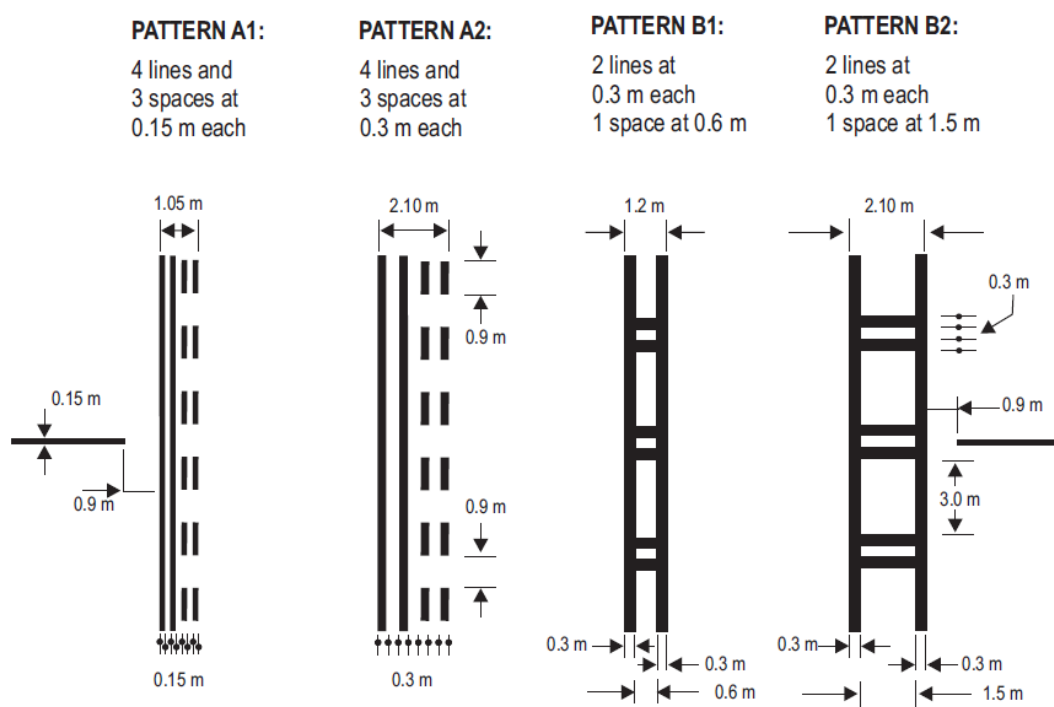
Figure 5-8. Runway-holding position markings
