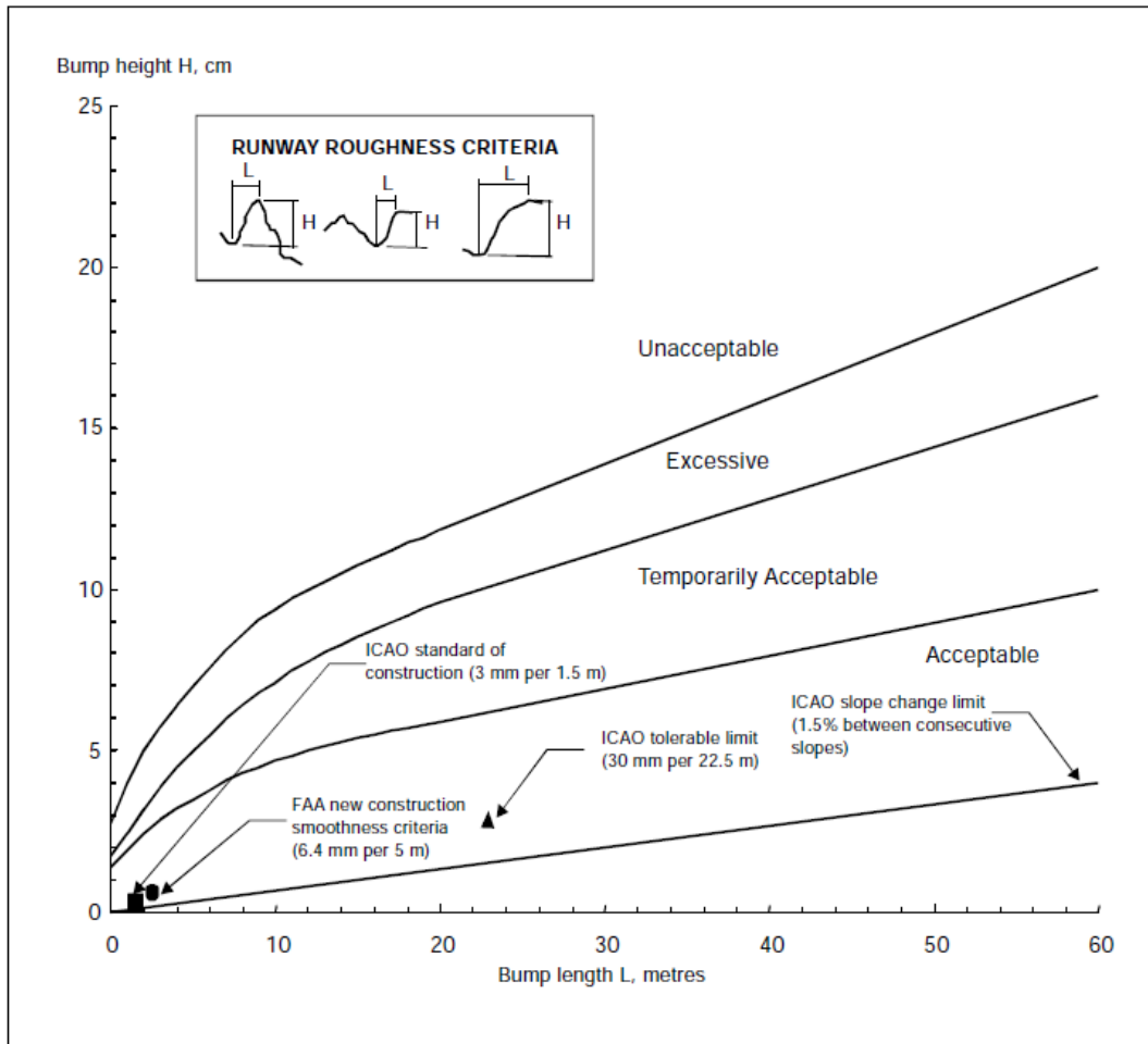
Figure A-3. Comparison of roughness criteria
