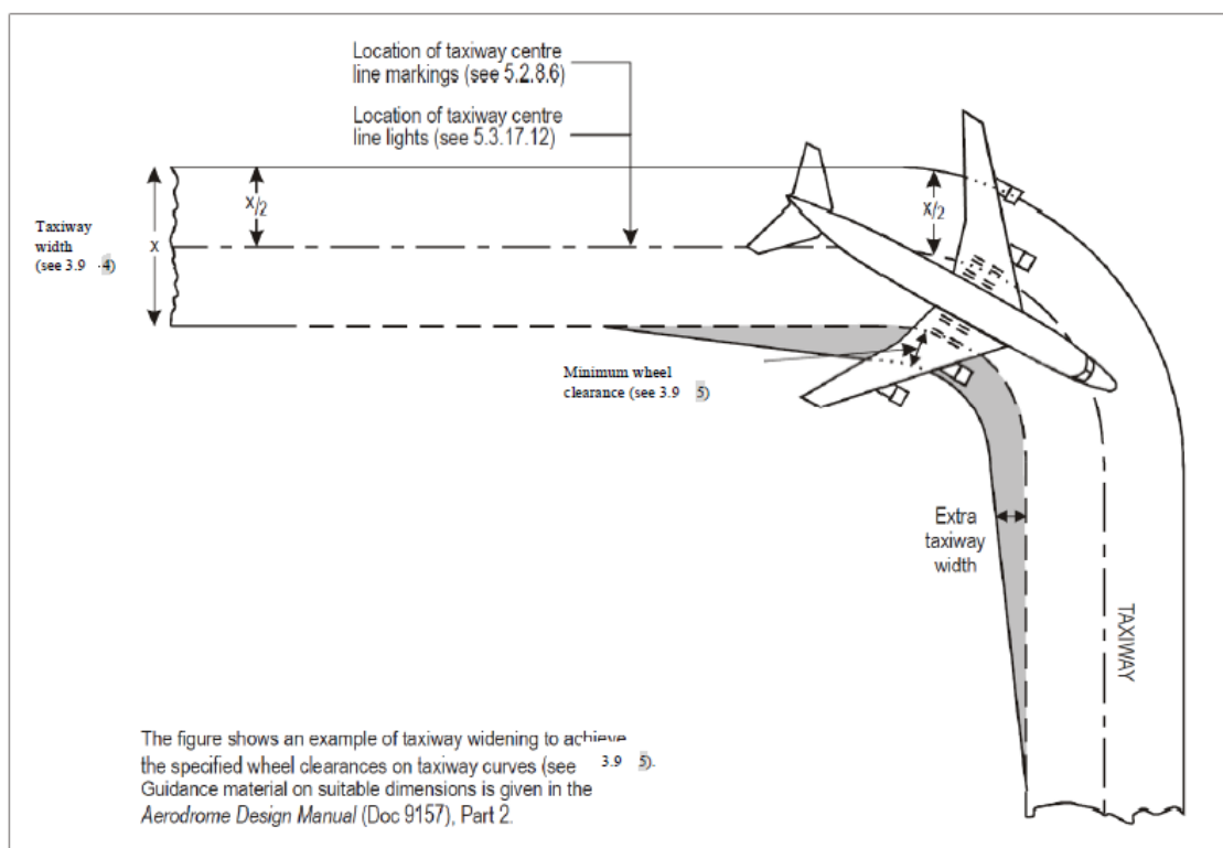
Figure 3-2. Taxiway Curve
