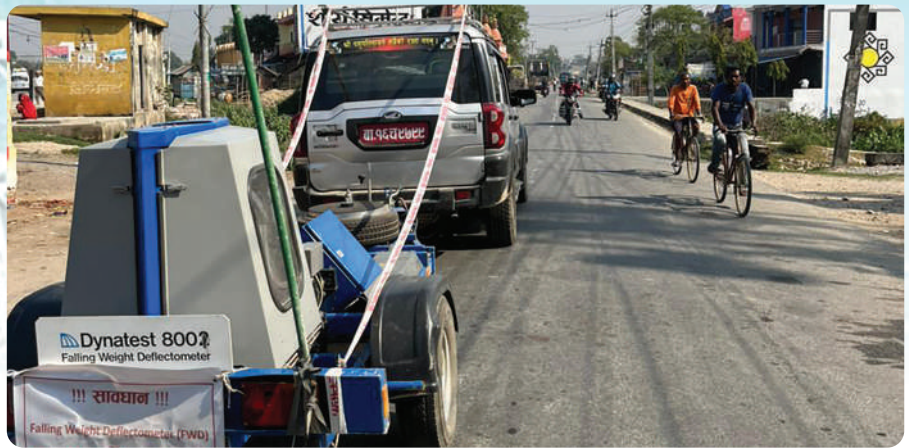
The deflection of road pavement at Kanchanpur in Saptari district being measured using FWD equipment on 29 March 2023.
