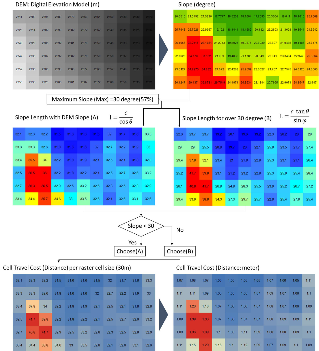
Figure 5: Flowchart for calculating Cost Distance
