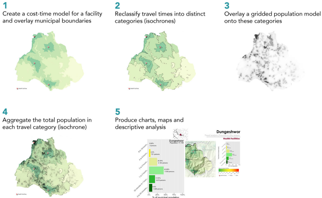
Figure 10: Analysis process for calculating population coverage by administrative unit
