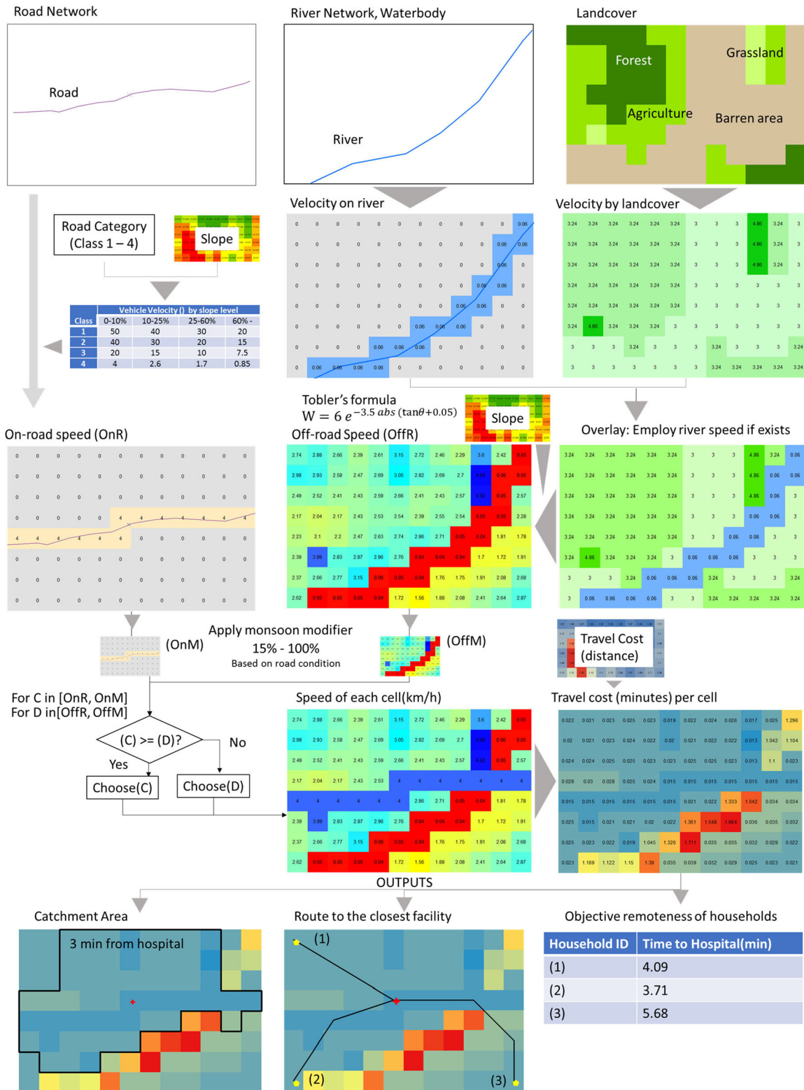
Figure 6: Flowchart for calculating Travel Time by Cost Distance
