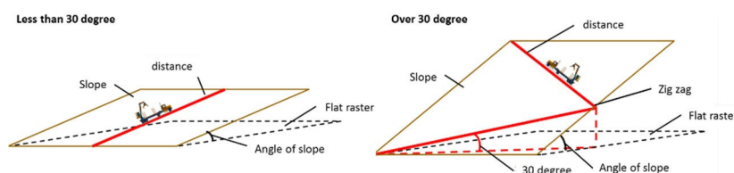
Figure 4: Zigzag route calculation
