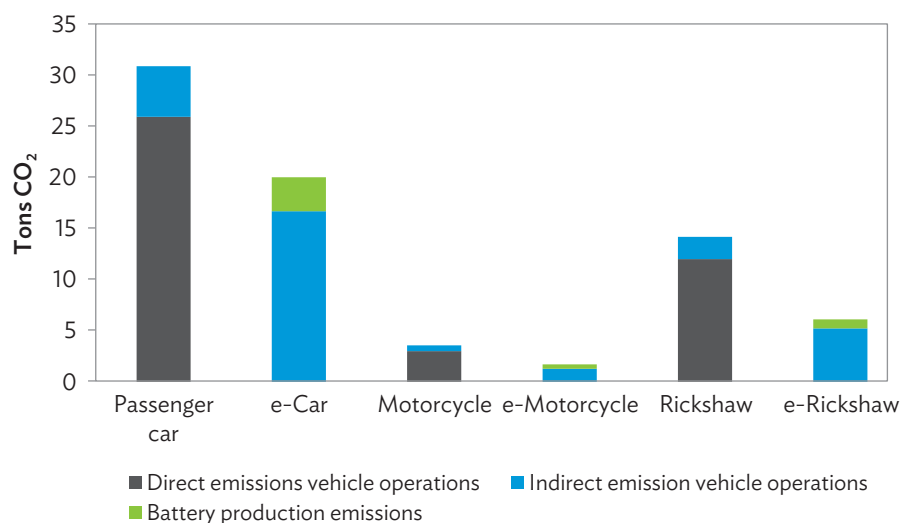
Figure 30: Greenhouse Gas Emissions Operations—Battery Cars, Motorcycles, and Rickshaws
