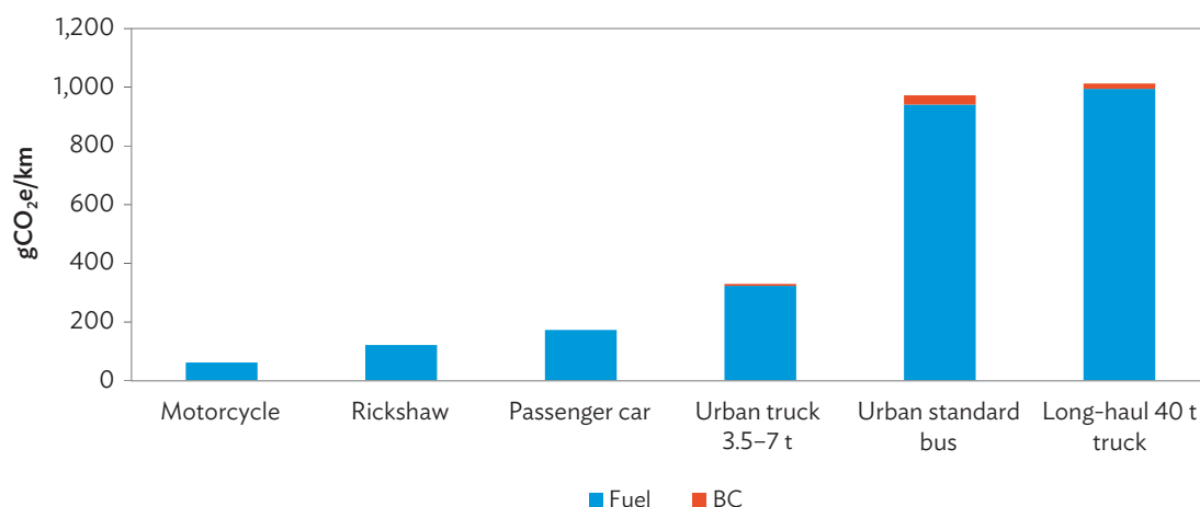
Figure 22: Average Tank-to-Wheel Greenhouse Gas Emissions of Standard Vehicle Categories (gCO 2 e/km)
