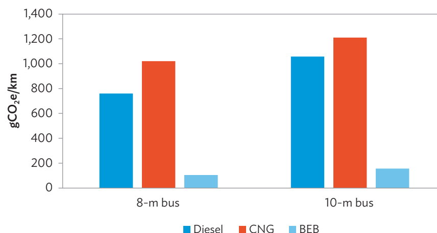
Figure 56: Greenhouse Gas Emissions—8-Meter and 10–12-Meter Urban Buses (gCO 2 e/km)
