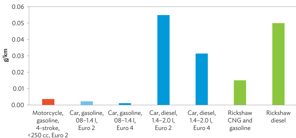
Figure 33: Particulate Matter Emissions—Light Vehicles (g/km)
