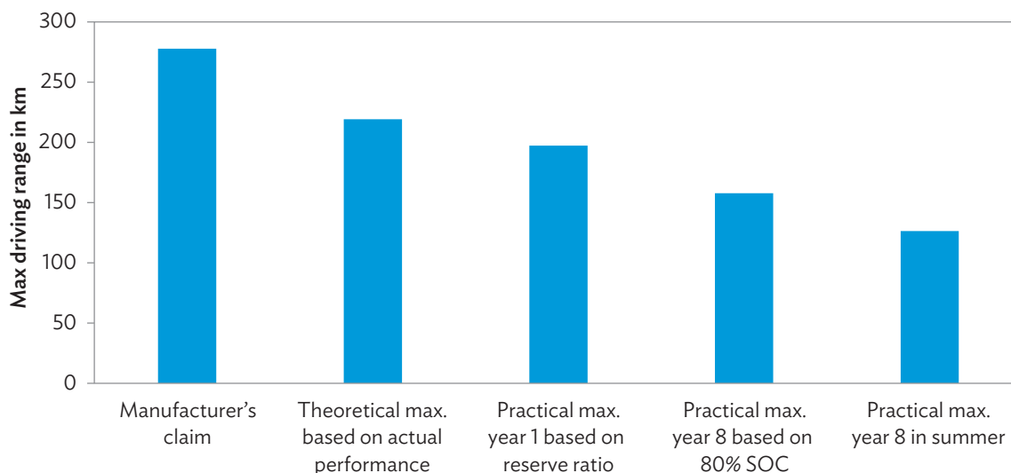
Figure 8: Maximum Driving Range of 12-Meter Battery Electric Buses with 250 Kilowatt-Hour Battery Pack
