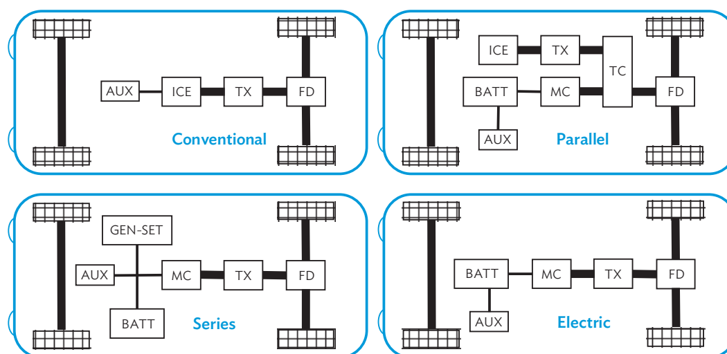
Figure 4: System Diagram—Conventional, Hybrid, and Electric Vehicle
