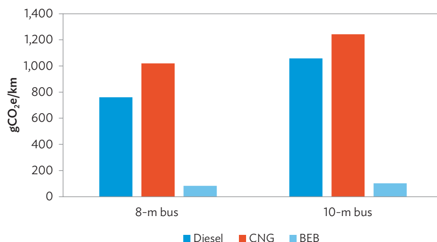
Figure 55: Greenhouse Gas Emissions—8-Meter and 10-Meter Urban Buses in Georgia (gCO 2 e/km)
