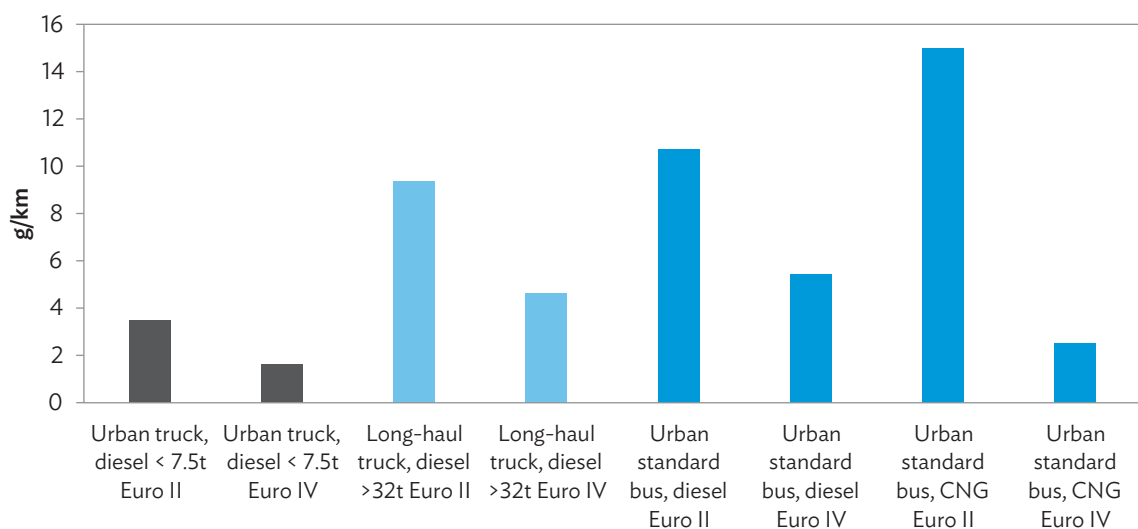
Figure 32: Nitrogen Oxide Emissions—Heavy Vehicles (g/km)
