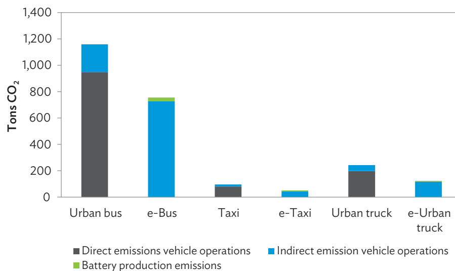
Figure 29: Greenhouse Gas Emissions Operations—Battery Buses, Urban Trucks, and Taxis
