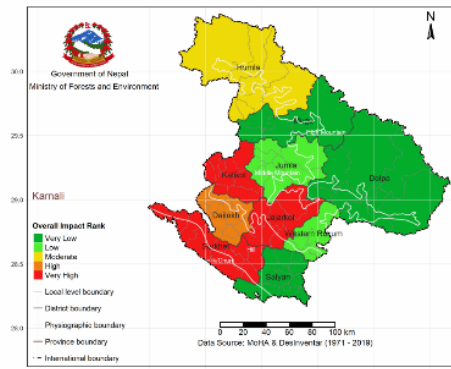
Overall Impact Rank in Karnali Province
