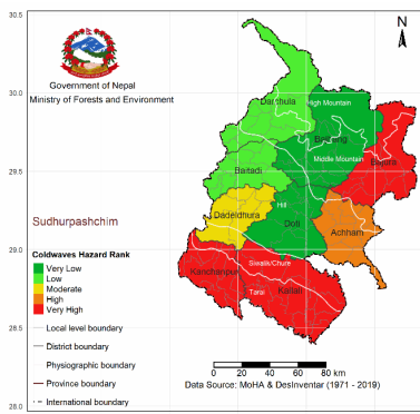
Coldwaves Hazard Rank in Sudurpashchim Province
