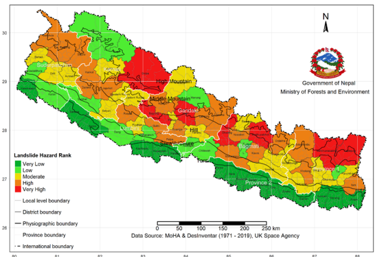
Landslide Hazard Rank
