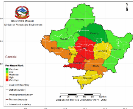
Fire Hazard Rank in Gandaki Province
