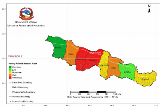
Heavy Rainfall Hazard Rank in Province 2
