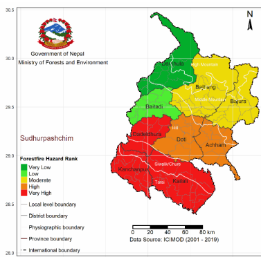
Forestfire Hazard Rank in Sudurpashchim Province
