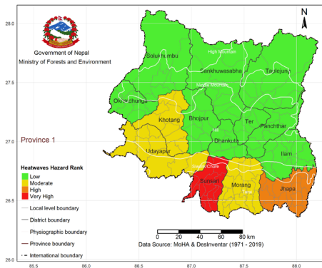
Heatwaves Hazard Rank in Province 1
