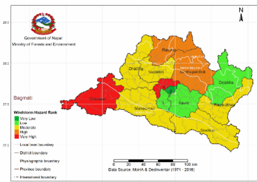
Windstorm Hazard Rank in Bagmati Province
