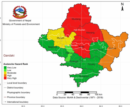
Avalanche Hazard Rank in Gandaki Province
