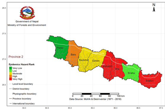
Epidemics Hazard Rank in Province 2
