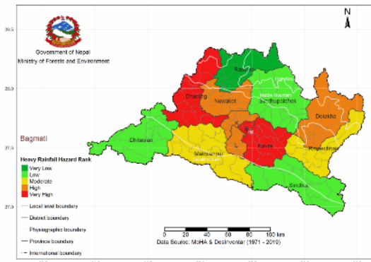
Heavy Rainfall Hazard Rank in Bagmati Province
