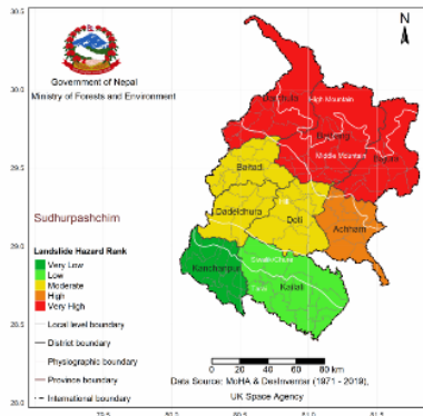
Landslide Hazard Rank in Sudurpashchim Province
