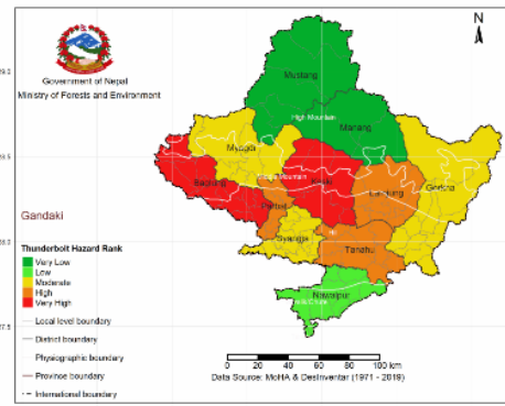
Thunderbolt Hazard Rank in Gandaki Province
