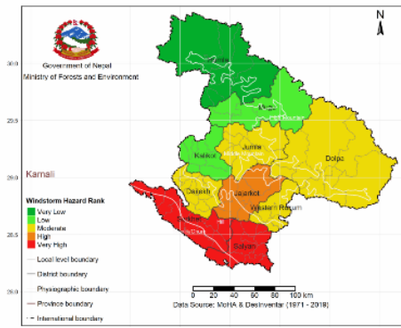
Windstorm Hazard Rank in Karnali Province
