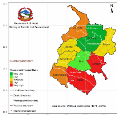
Thunderbolt Hazard Rank in Sudurpashchim Province
