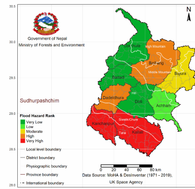
Flood Hazard Rank in Sudurpashchim Province
