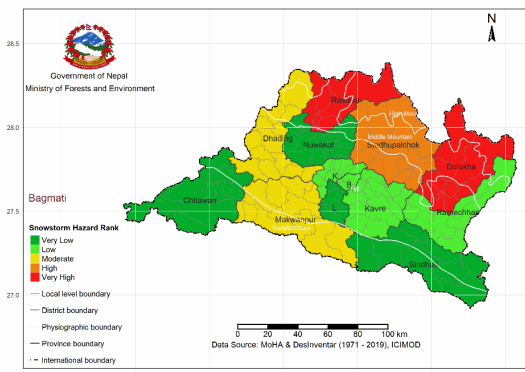
Snowstorm Hazard Rank in Bagmati Province
