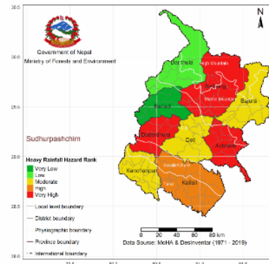
Heavy Rainfall Hazard Rank in Sudurpashchim Province
