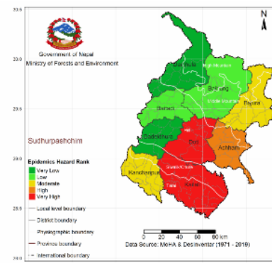
Epidemics Hazard Rank in Sudurpashchim Province
