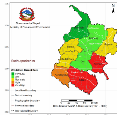
Windstorm Hazard Rank in Sudurpashchim Province
