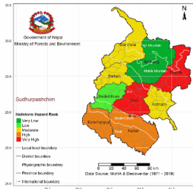
Hailstorm Hazard Rank in Sudurpashchim Province
