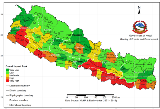
Overall Impact Rank
