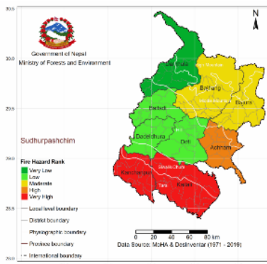
Fire Hazard Rank in Sudurpashchim Province
