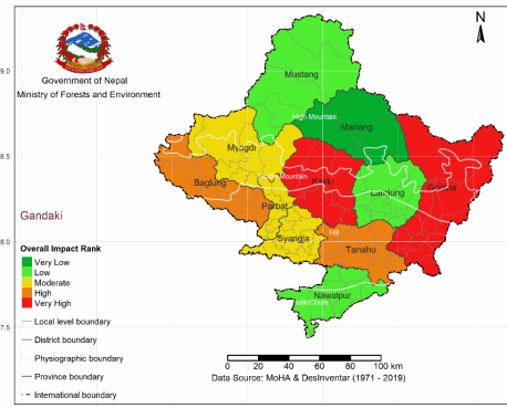
Overall Impact Rank in Gandaki Province
