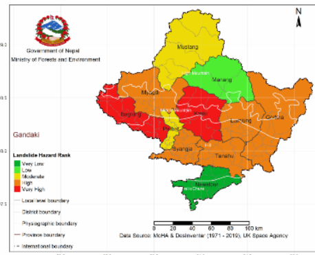
Landslide Hazard Rank in Gandaki Province
