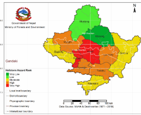
Hailstorm Hazard Rank in Gandaki Province
