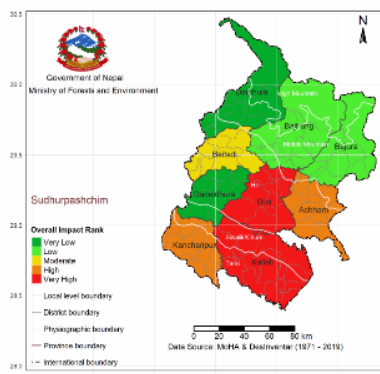
Overall Impact Rank in Sudurpashchim Province
