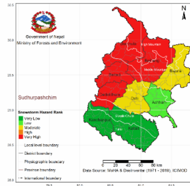
Snowstorm Hazard Rank in Sudurpashchim Province
