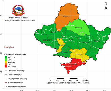
Coldwaves Hazard Rank in Gandaki Province
