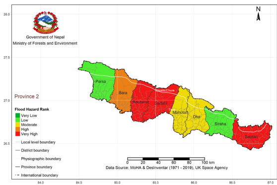
Flood Hazard Rank in Province 2
