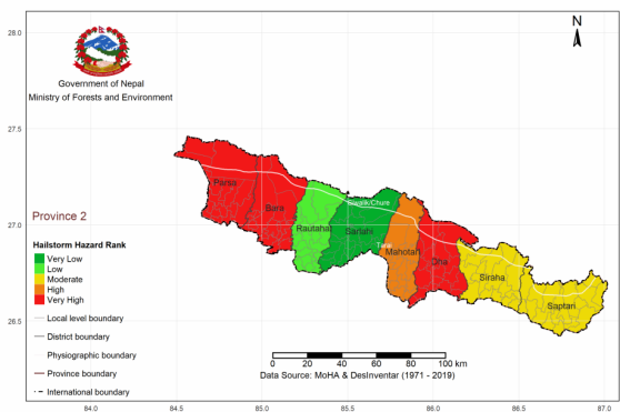
Hailstorm Hazard Rank in Province 2
