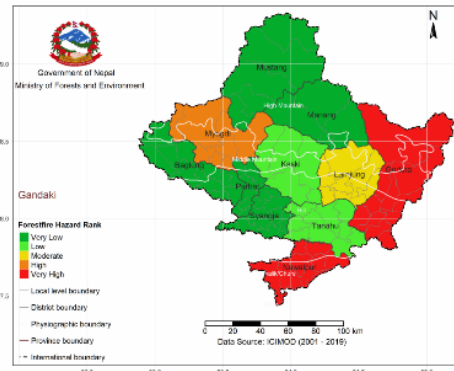
Forestfire Hazard Rank in Gandaki Province
