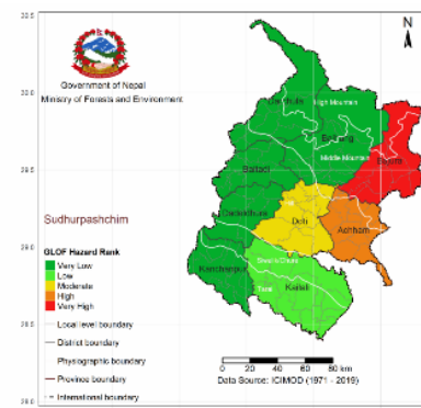
GLOF Hazard Rank in Sudurpashchim Province
