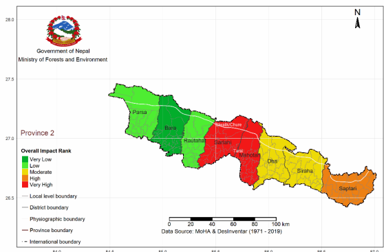
Overall Impact Rank in Province 2
