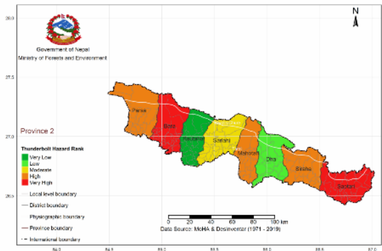
Thunderbolt Hazard Rank in Province 2
