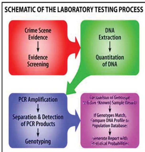
Fig 3: Steps in DNA analysis
