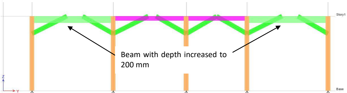
Figure 6: Beams with depth increased to 200 mm
