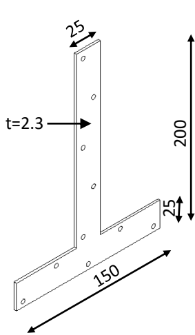
'T' shape metal plate
